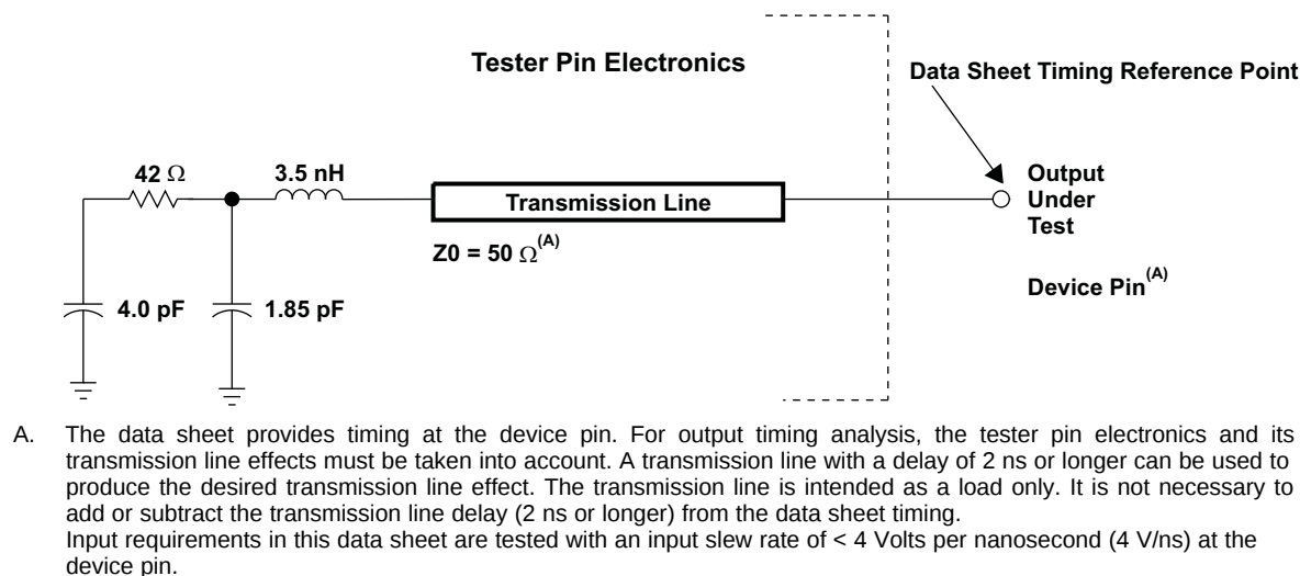
Figure 6-9. 3.3-V Test Load Circuit
