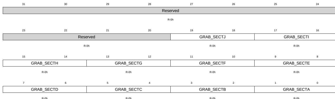
Figure 1-111. Z1_GRABSECTR Register
