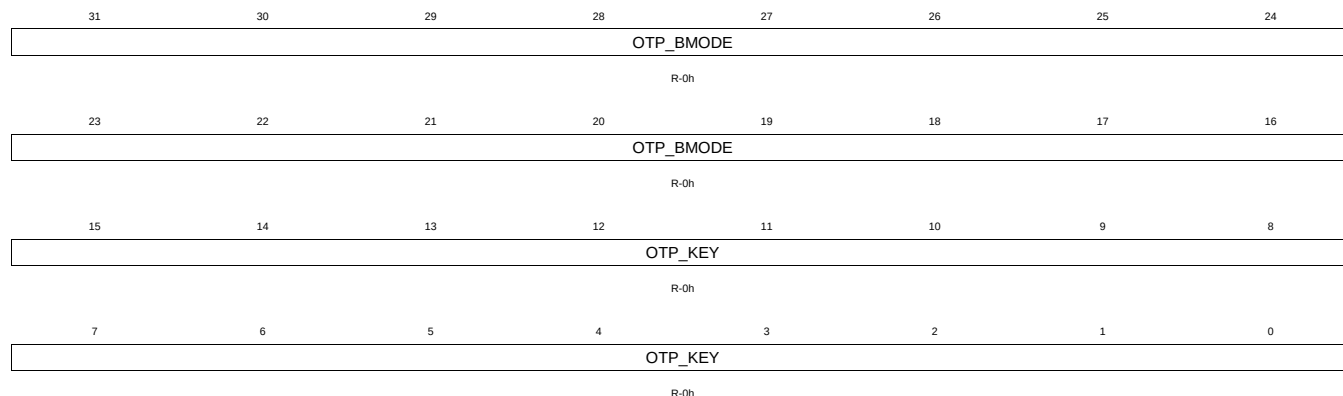
Figure 1-99. Z2_BOOTMODE Register
