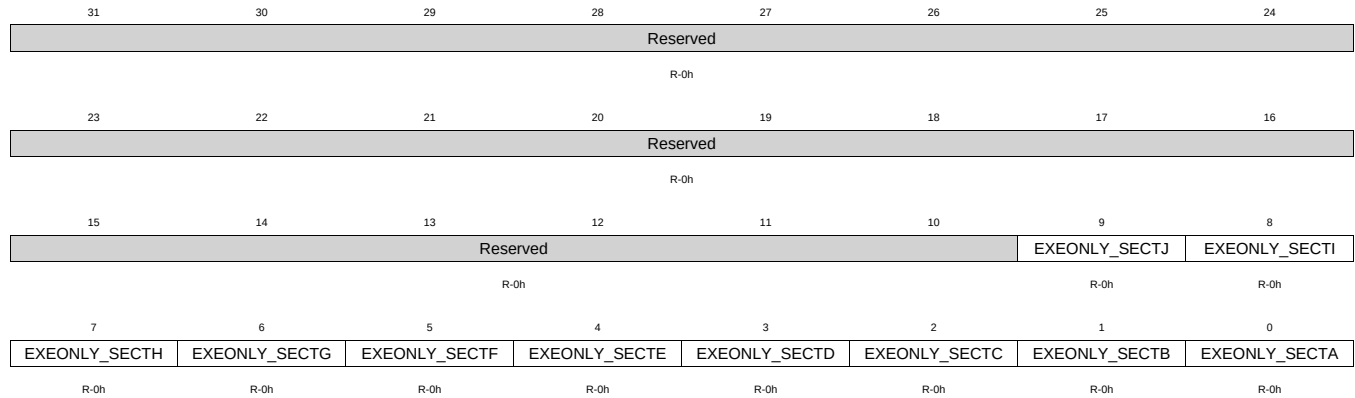
Figure 1-113. Z1_EXEONLYSECTR Register
