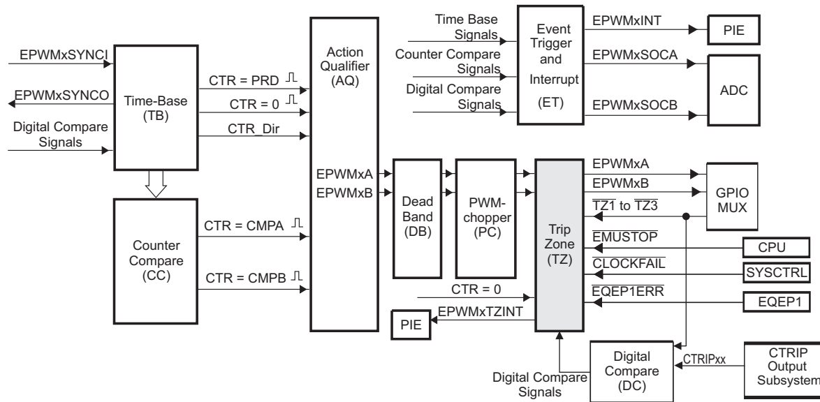
Figure 3-36. Trip-Zone Submodule
