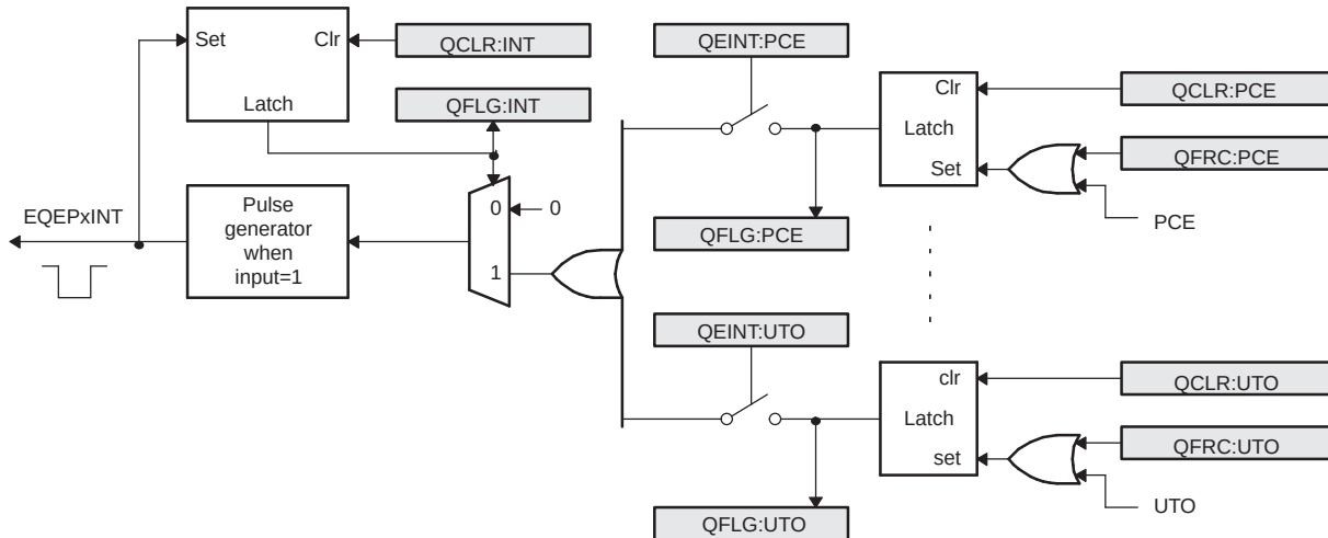
Figure 5-20. EQEP Interrupt Generation
