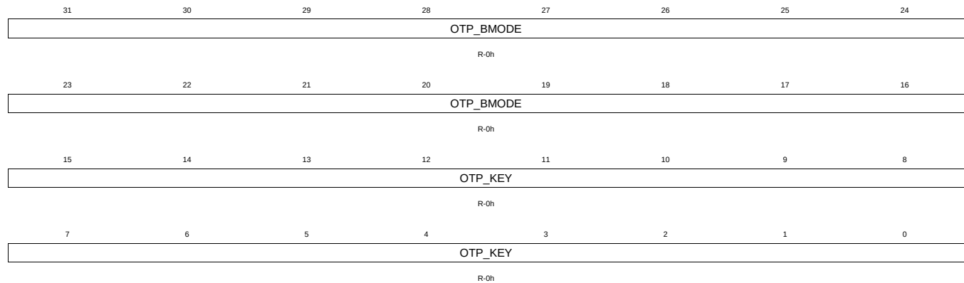
Figure 1-96. Z1_BOOTMODE Register
