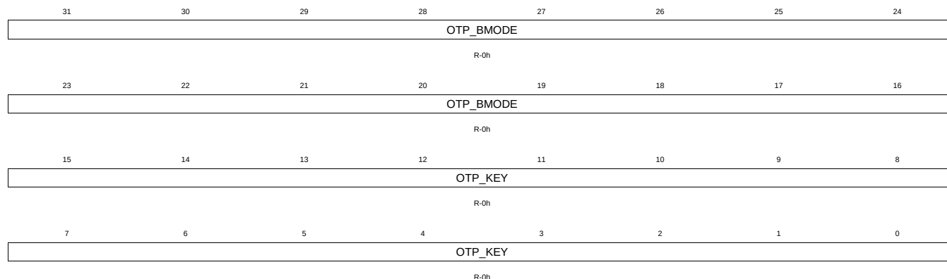
Figure 1-117. Z2_BOOTMODE Register
