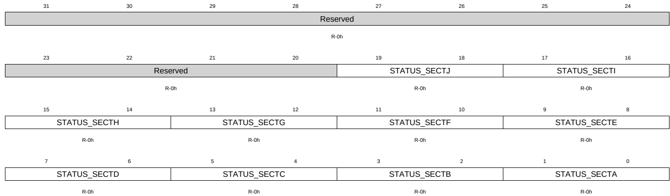
Figure 1-101. SECTSTAT Register
