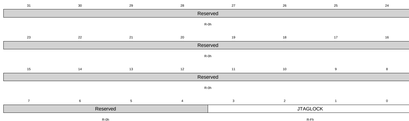
Figure 1-104. Z1_OTPSECLOCK Register
