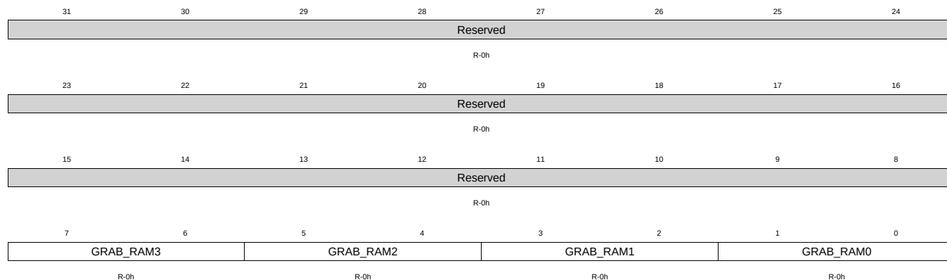
Figure 1-112. Z1_GRABRAMR Register
