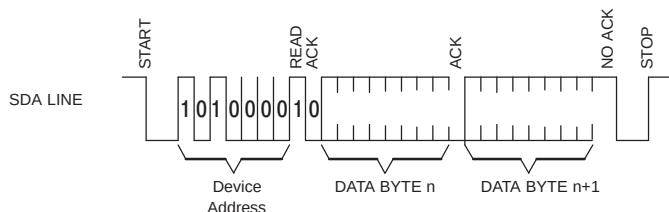
Figure 2-25. Sequential Read
