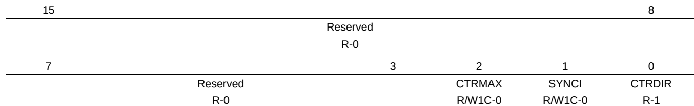
Figure 3-74. Time-Base Status Register (TBSTS)
