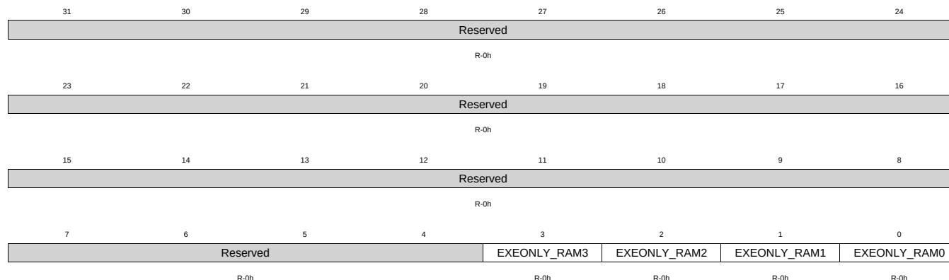
Figure 1-126. Z2_EXEONLYRAMR Register
