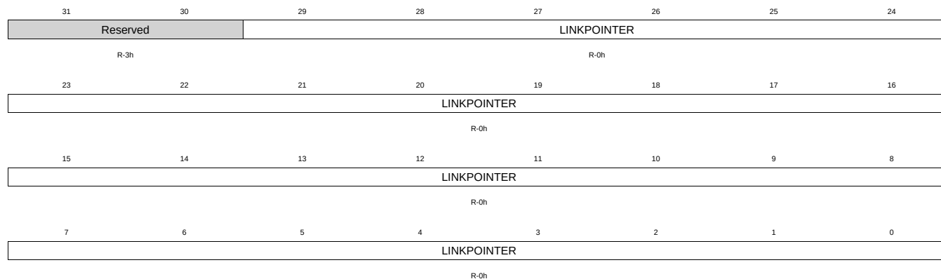
Figure 1-97. Z2_LINKPOINTER Register
