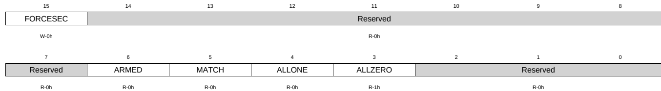
Figure 1-110. Z1_CR Register
