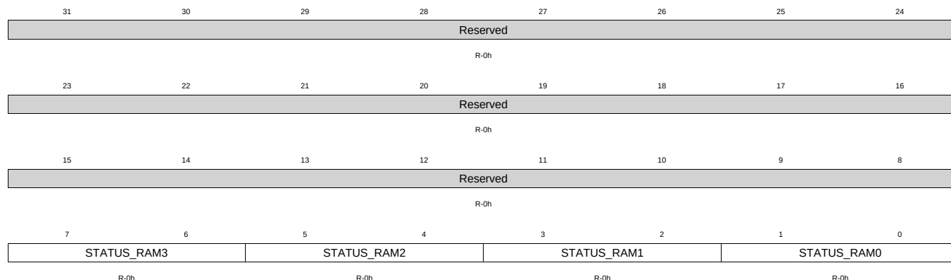
Figure 1-102. RAMSTAT Register
