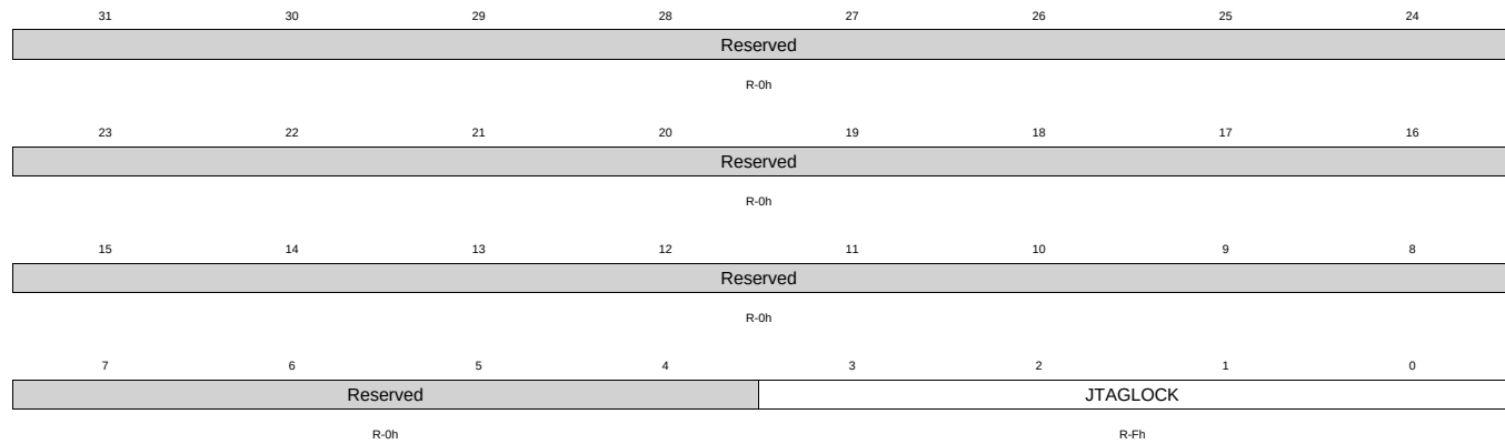
Figure 1-98. Z2_OTPSECLOCK Register
