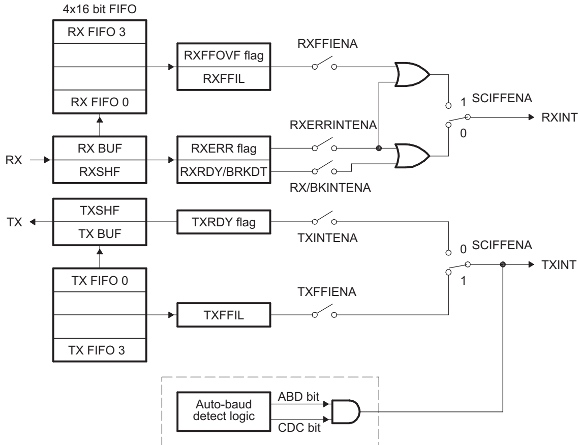
Figure 11-10. SCI FIFO Interrupt Flags and Enable Logic
