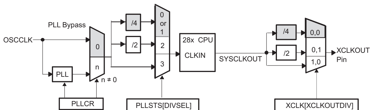
Figure 1-30. XCLKOUT Generation
