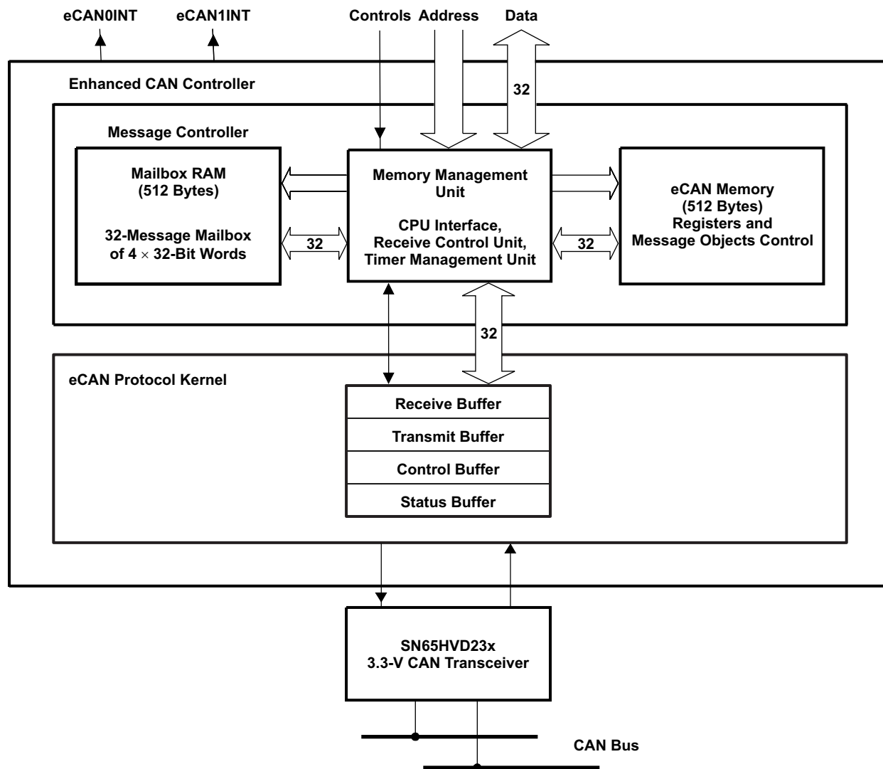
Figure 6-34. eCAN Block Diagram and Interface Circuit
