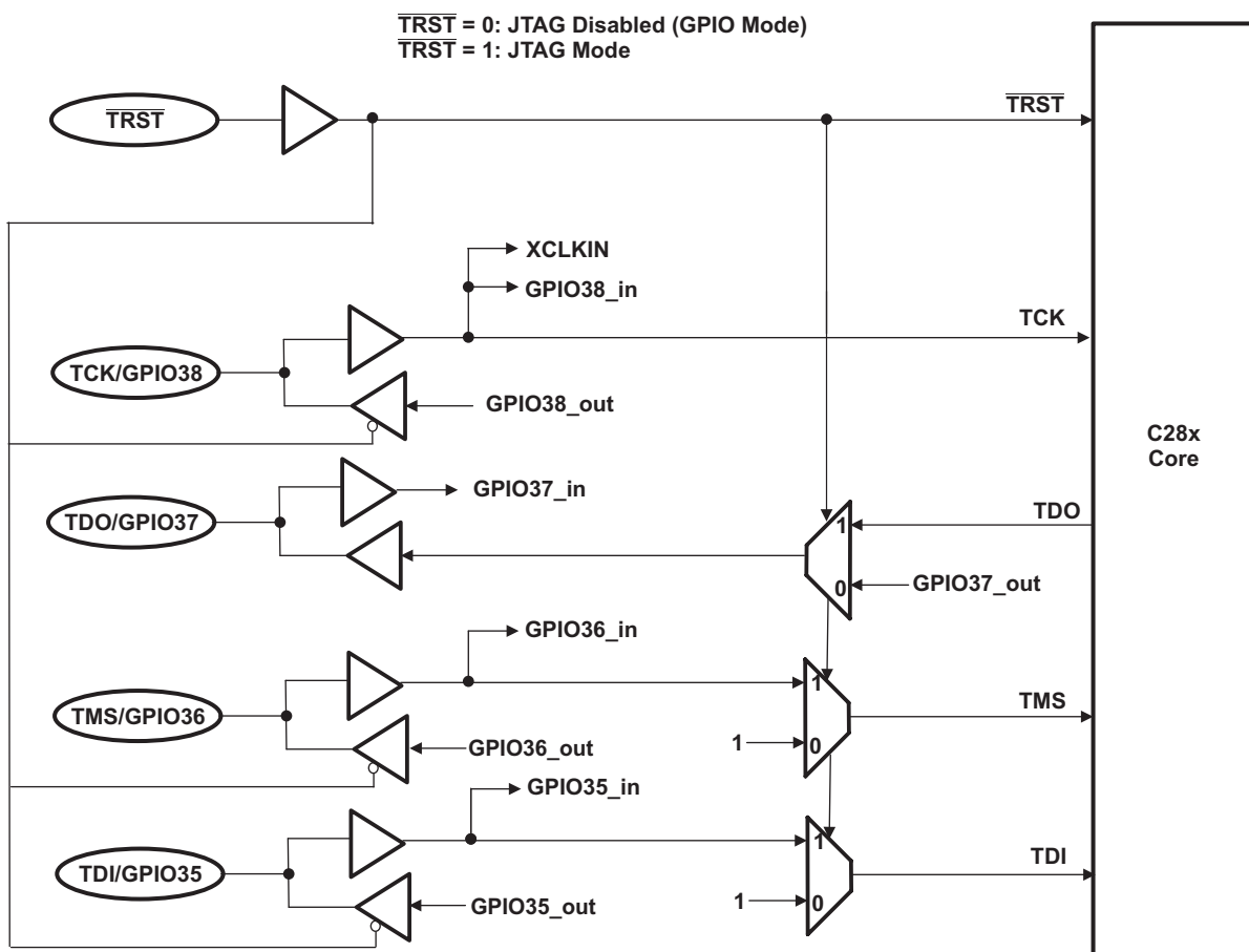
Figure 6-42. JTAG/GPIO Multiplexing
