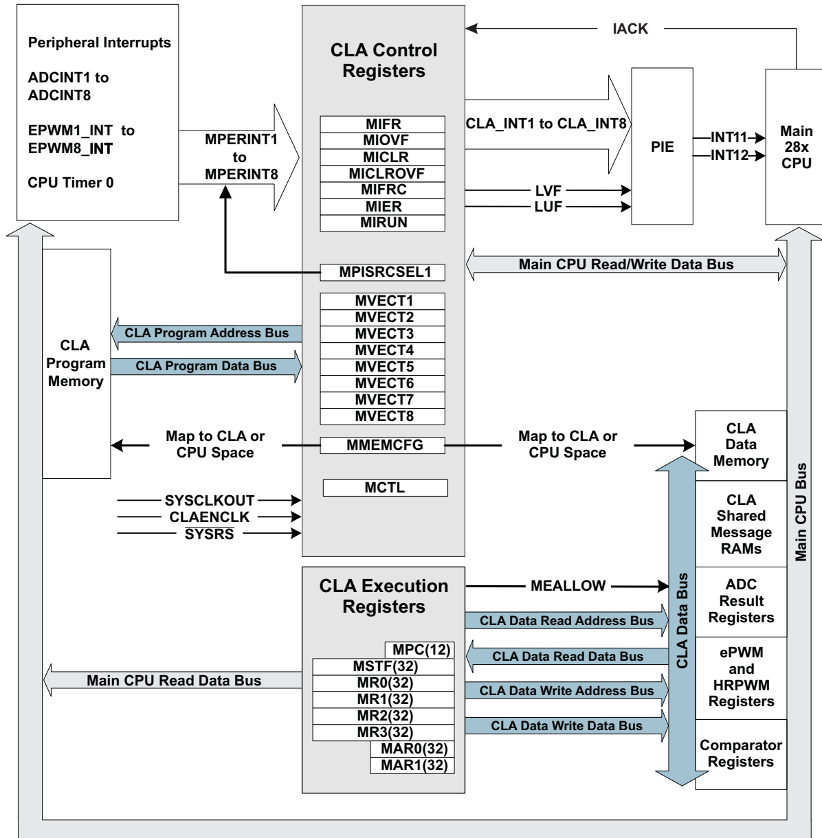
Figure 6-15. CLA Block Diagram
