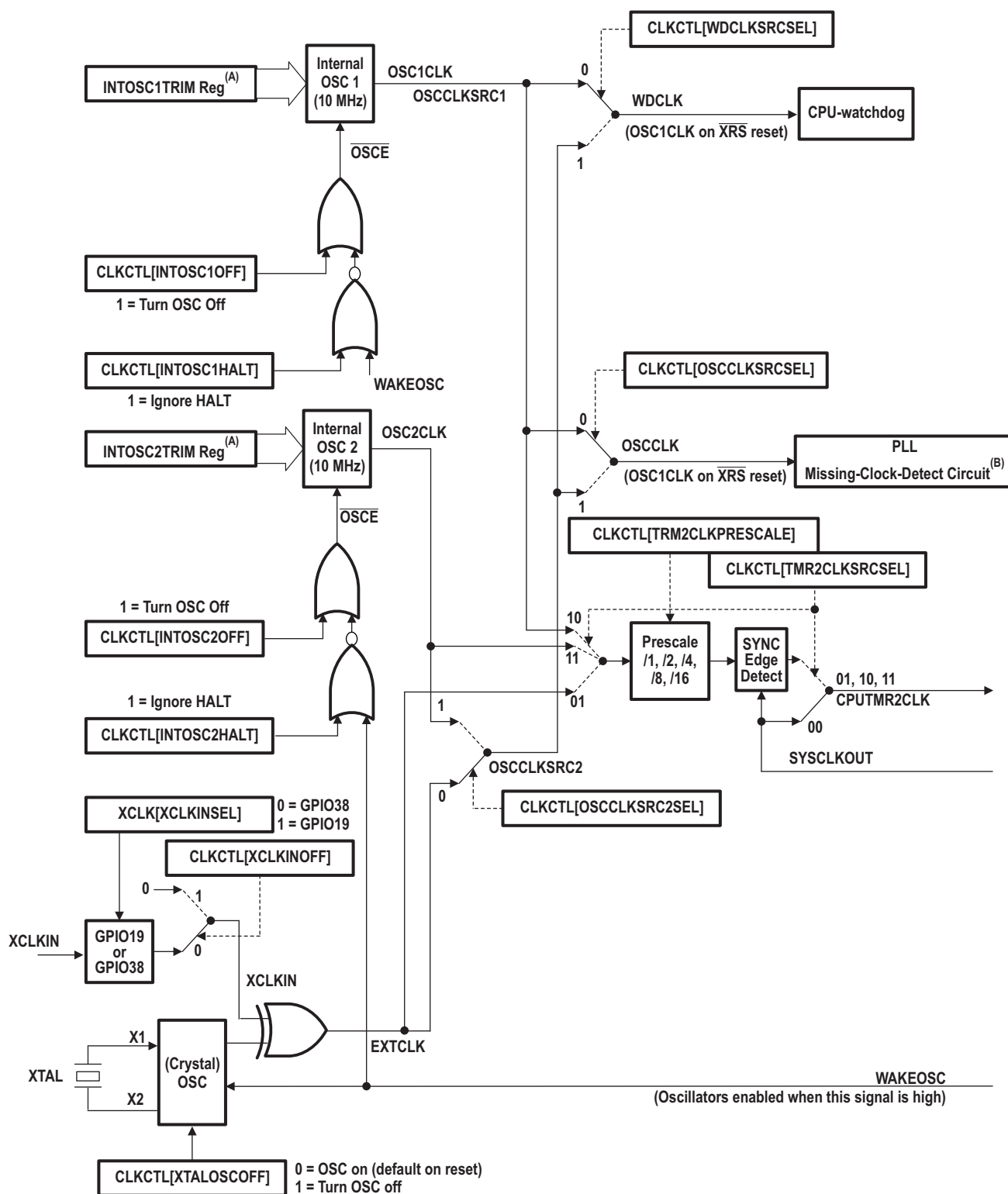
Figure 5-4. Clock Tree
