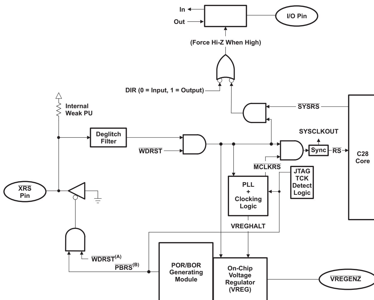
Figure 5-2. VREG + POR + BOR + Reset Signal Connectivity
