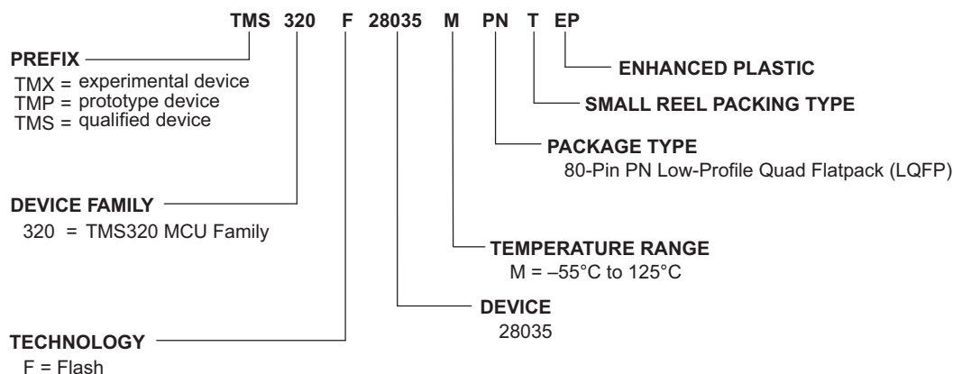
Figure 7-1. Device Nomenclature
