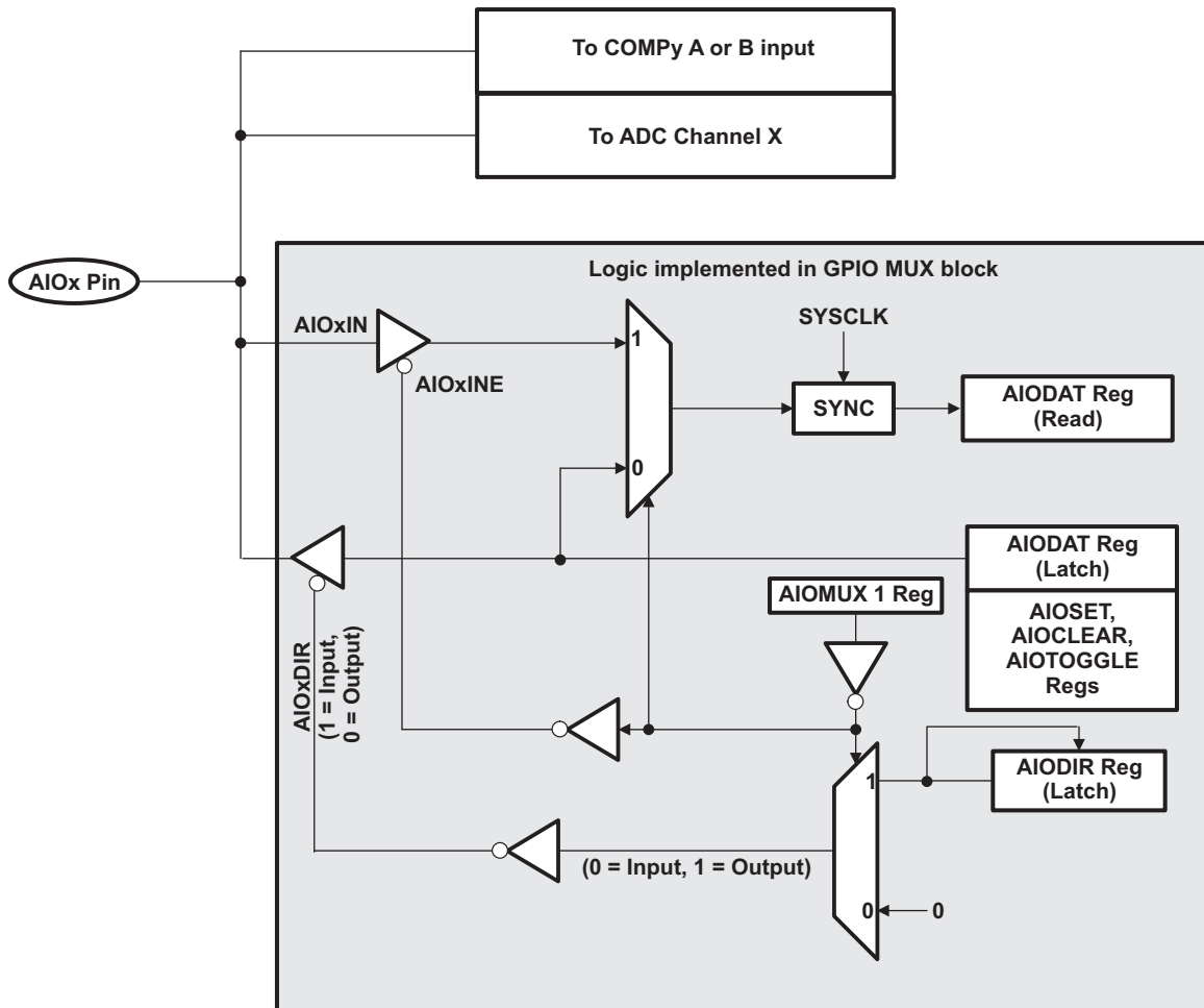
Figure 5-22. AlOx Pin Multiplexing
