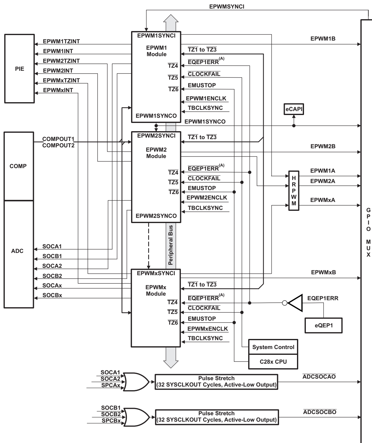
Figure 5-35. ePWM
