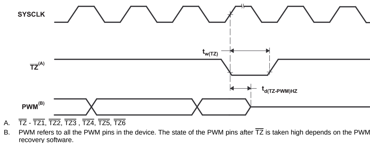
Figure 5-37. PWM Hi-Z Characteristics
