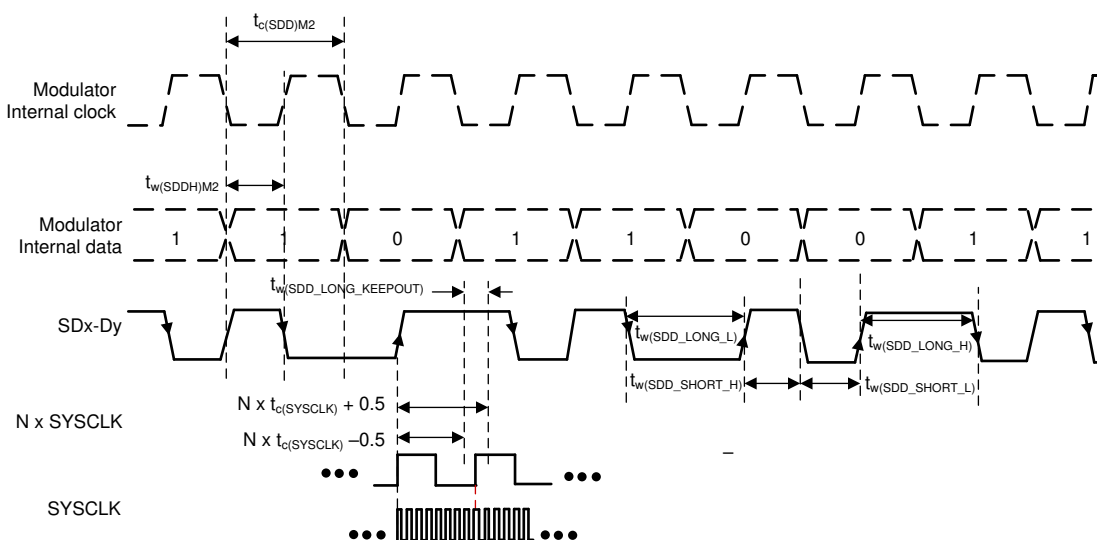
Figure 5-67. SDFM Timing Diagram – Mode 2
