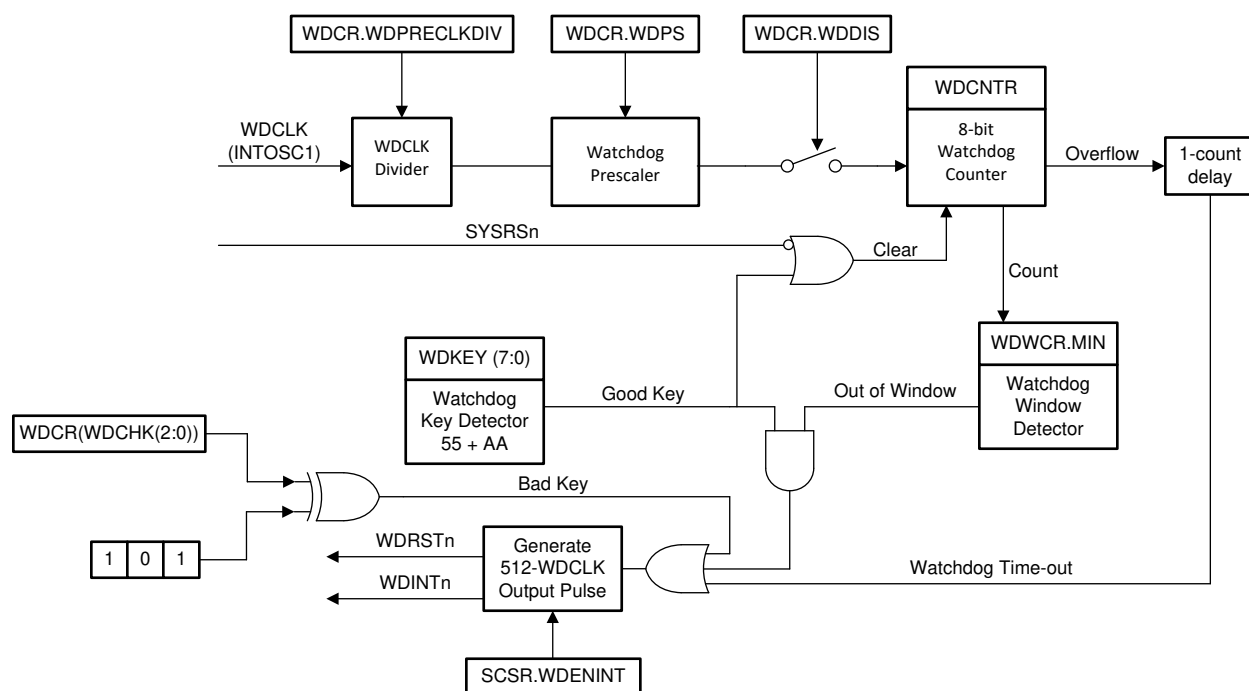
Figure 6-4. Windowed Watchdog
