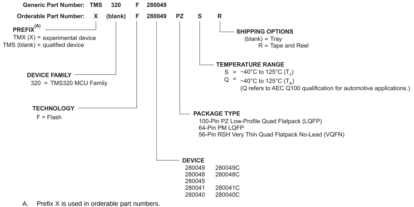
Figure 8-1. Device Nomenclature
