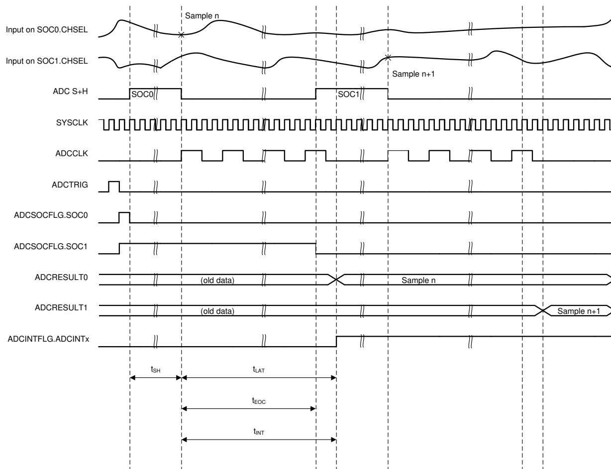
Figure 5-29. ADC Timings
