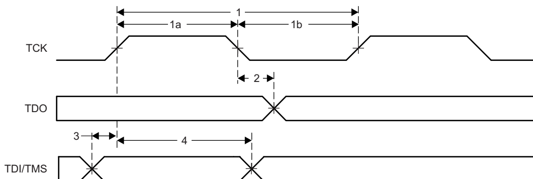
Figure 5-14. JTAG Timing
