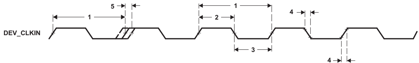
Figure 8-6. DEV_CLKIN Timing
