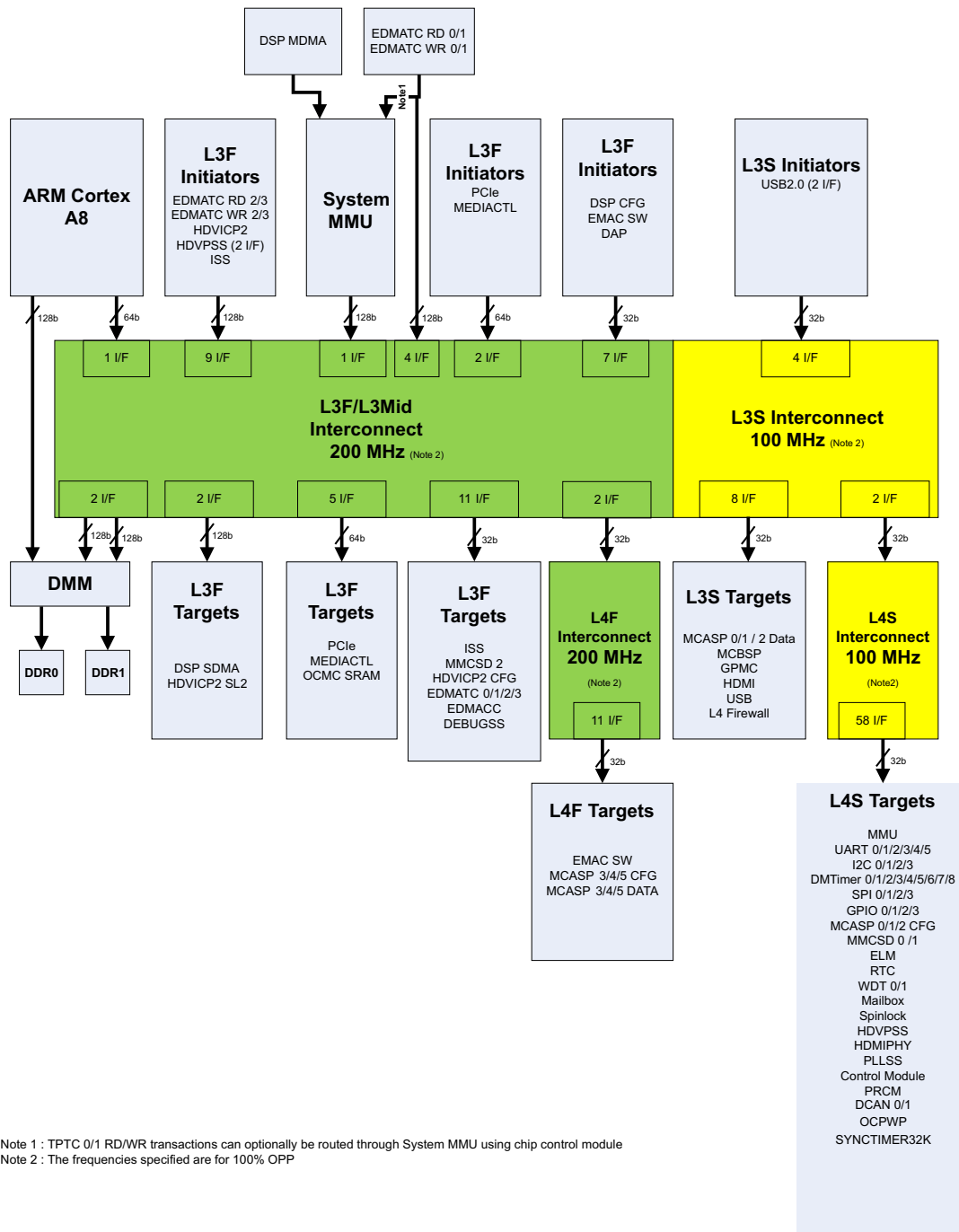
Figure 6-1. System Interconnect
