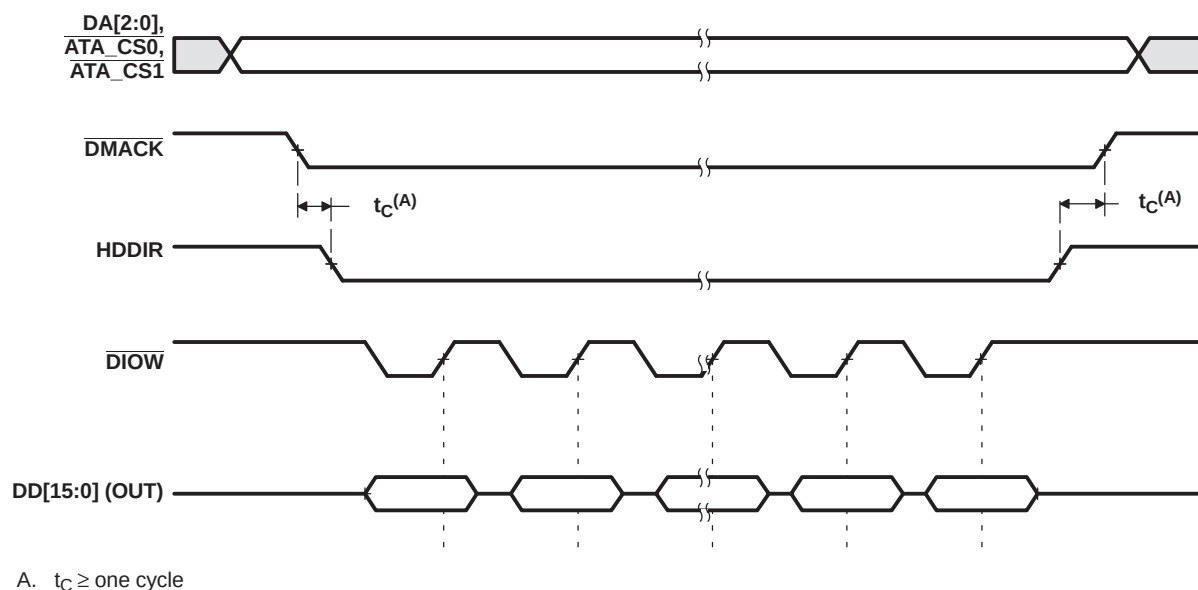
Figure 6-40. ATA/CF HDDIR Multiword DMA Write Transfer Timing
