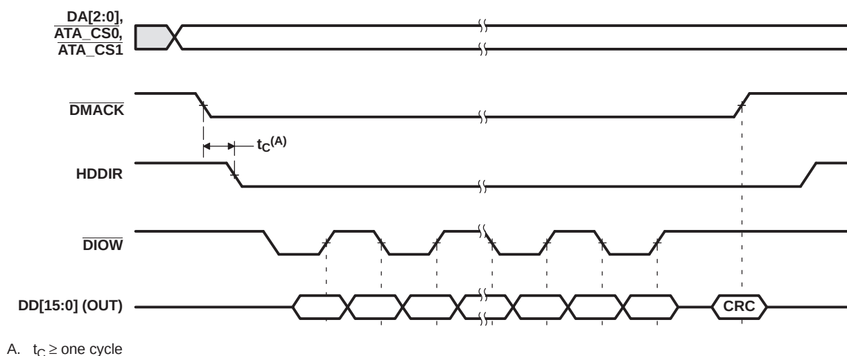
Figure 6-41. ATA/CF HDDIR Ultra DMA Write Transfer Timing
