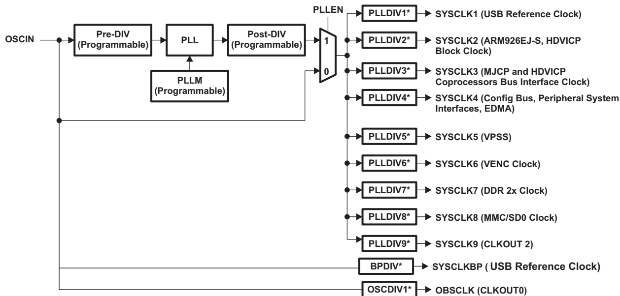
Figure 4-3. PLLC1 Configuration
