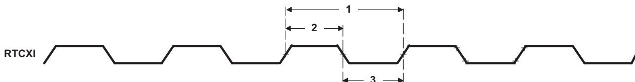
Figure 7-10. RTCXI Timing
