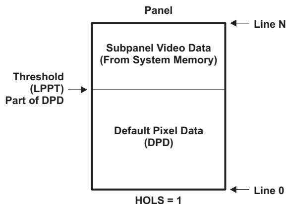
Figure 22-39. Subpanel Display: SPEN = 1, HOLs = 1
