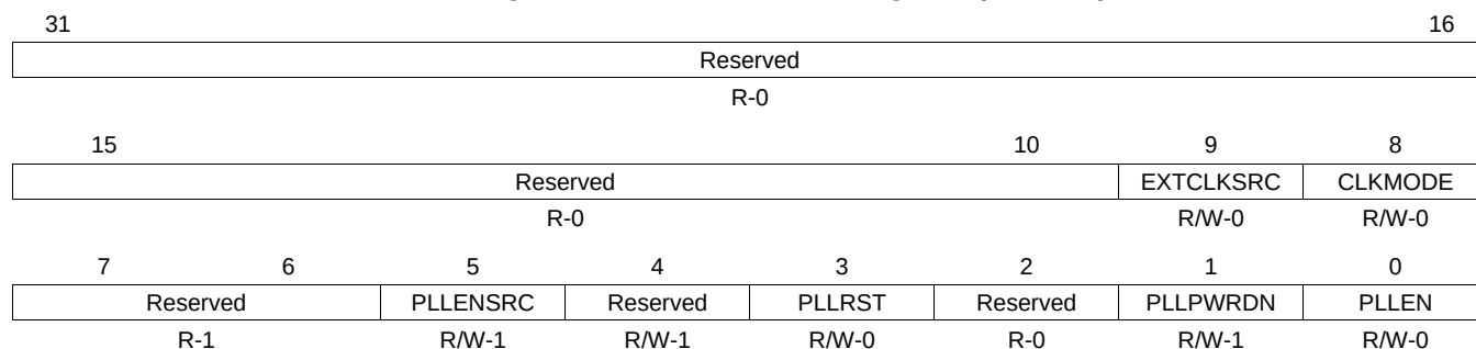
Figure 7-6. PLLC0 Control Register (PLLCTL)
