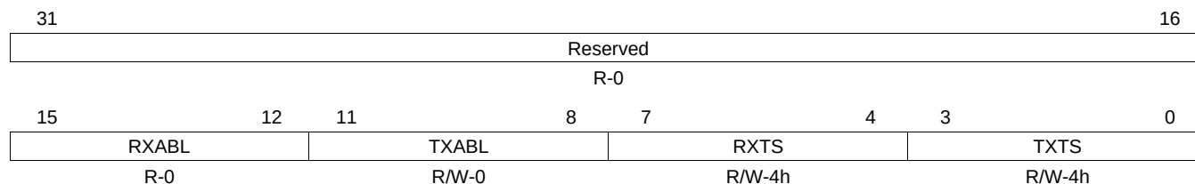
Figure 27-33. Port DMA Control Register (P0DMACR)
