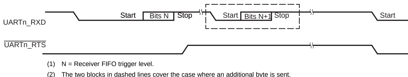
Figure 30-6. Autoflow Functional Timing Waveforms for UARTn_RTS
