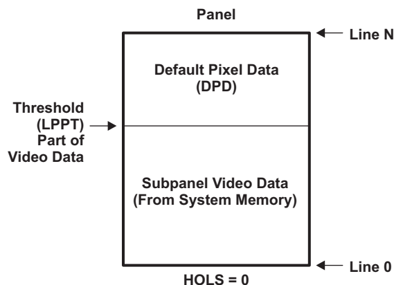
Figure 22-40. Subpanel Display: SPEN = 1, HOLs = 0
