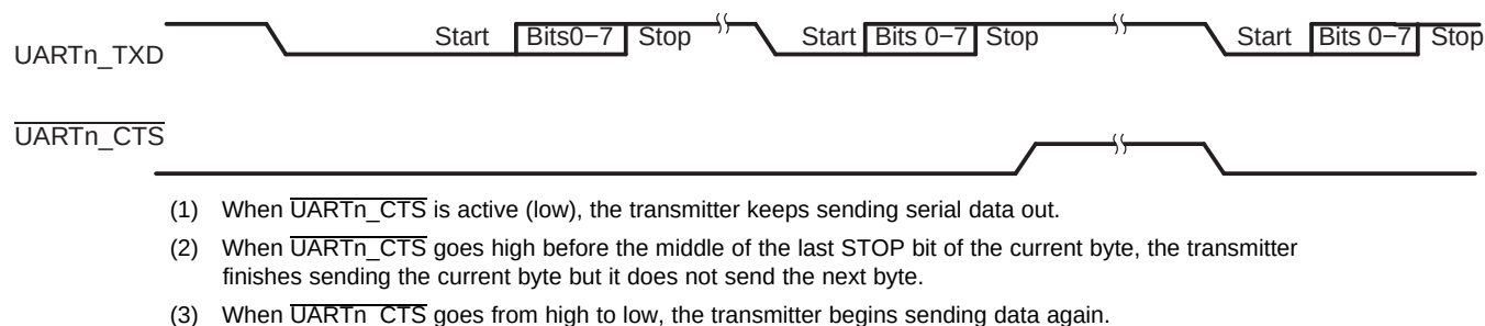
Figure 30-7. Autoflow Functional Timing Waveforms for UARTn_CTS
