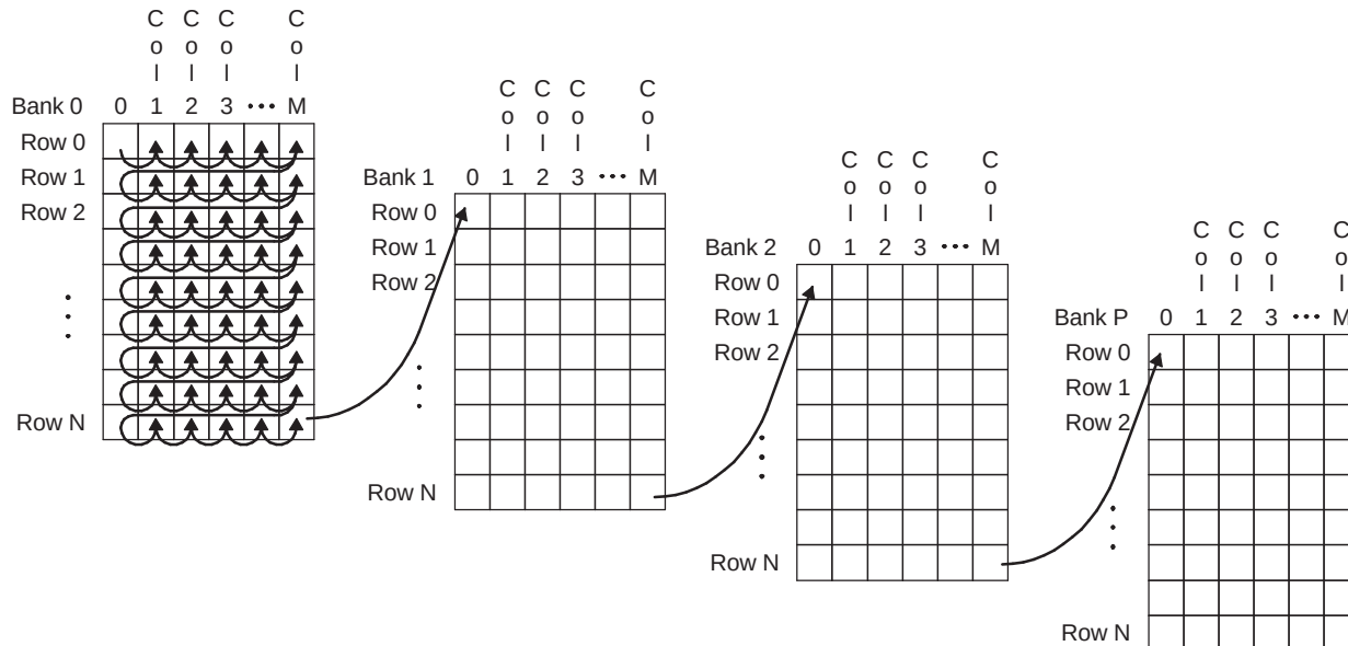
Figure 13-14. SDRAM Column, Row, Bank Access (IBANKPOS = 1)
