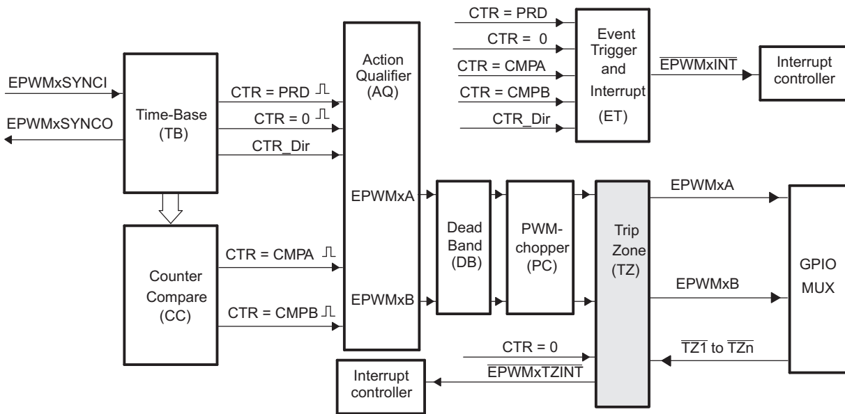
Figure 15-36. Trip-Zone Submodule
