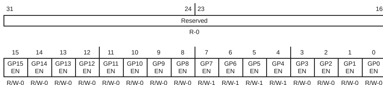
Figure 18. GPIO Enable Register (GPEN) [Hex Address: 01B0 0000]
