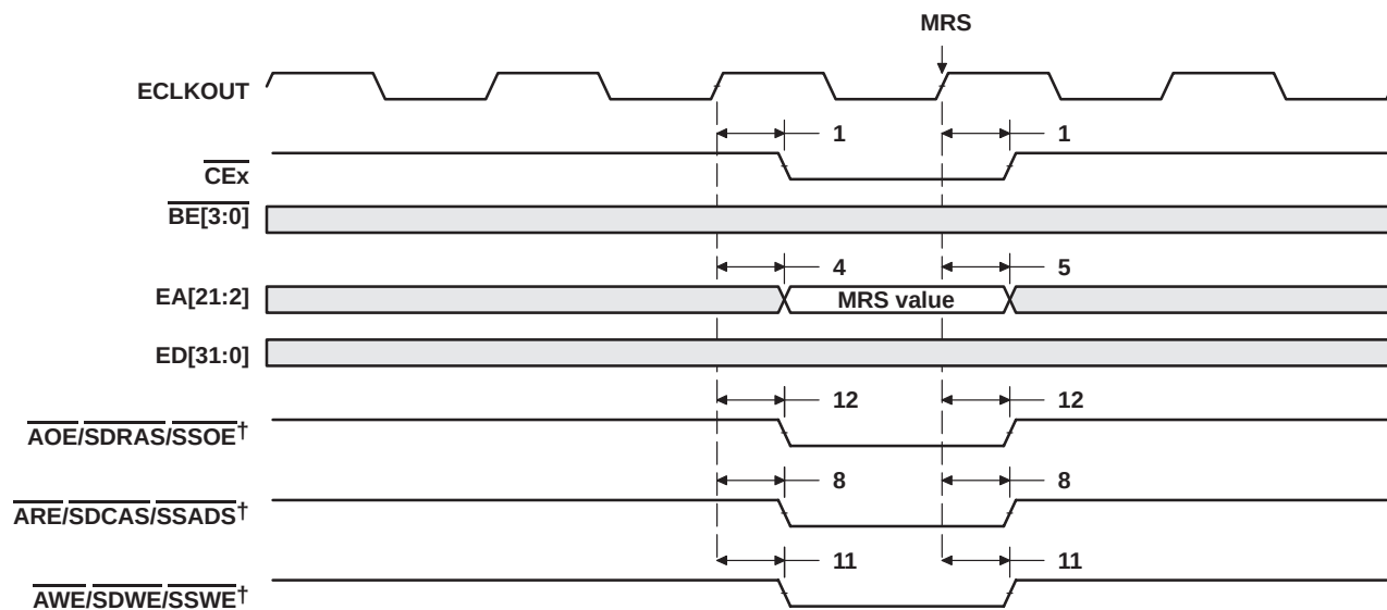
Figure 46. SDRAM MRS Command
