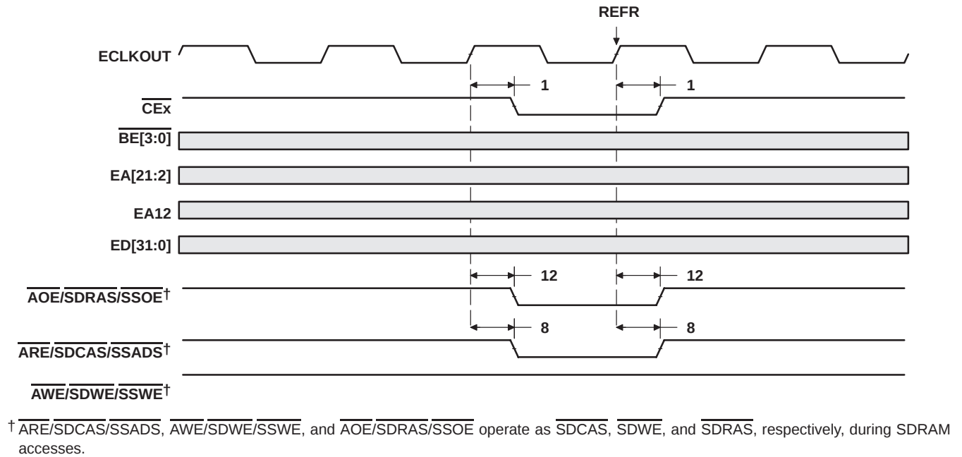
Figure 38. SDRAM REFR Command
