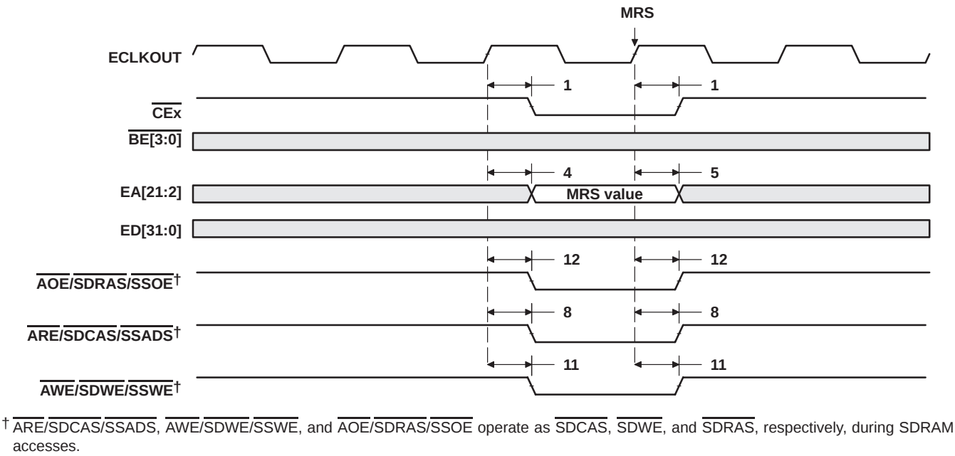
Figure 39. SDRAM MRS Command
