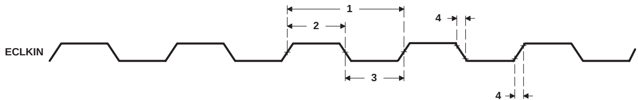
Figure 27. ECLKIN Timings
