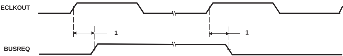
Figure 41. BUSREQ Timing
