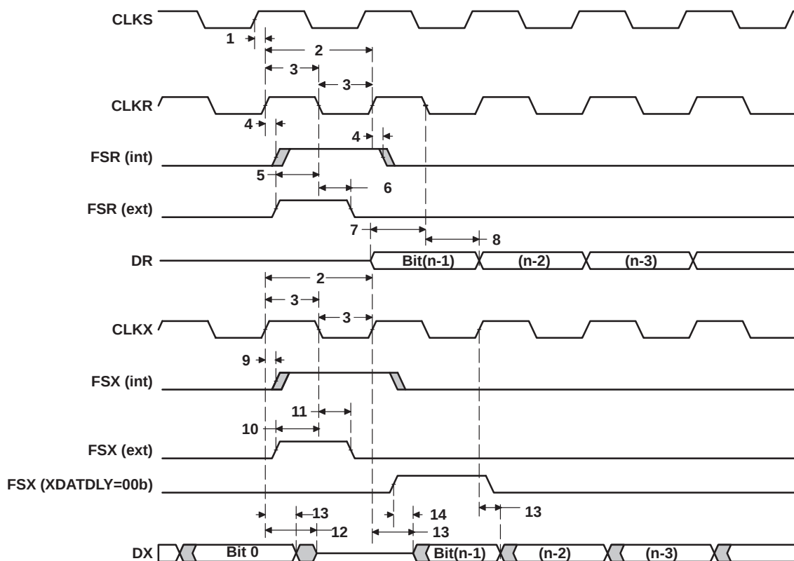
Figure 49. McBSP Timings
