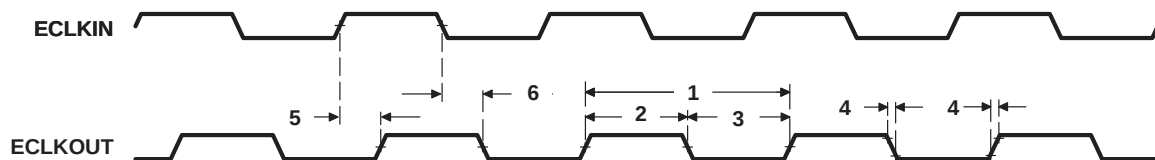
Figure 28. ECLKOUT Timings
