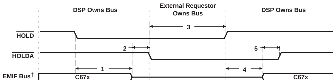
Figure 40. HOLD/HOLDA Timing
