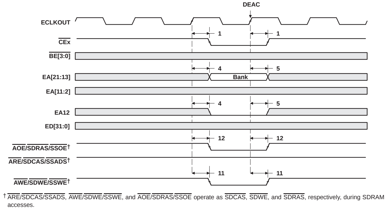
Figure 37. SDRAM DEAC Command
