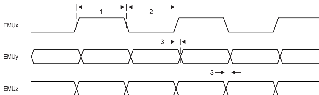
Figure 7-64 Trace Timing
