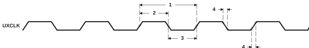
Figure 7-74. UXCLK Timing
