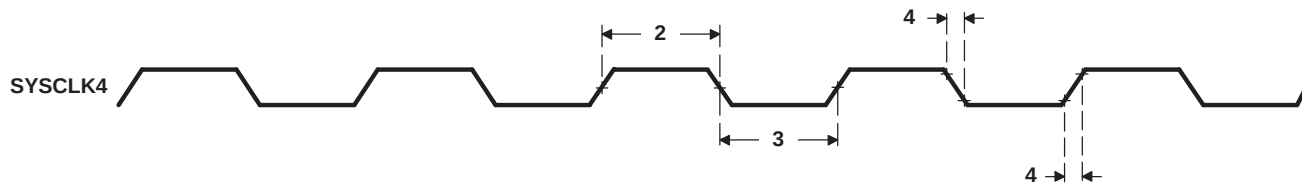
Figure 7-22. SYSCLK4 Timing
