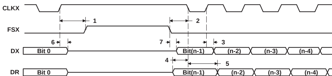
Figure 7-57. McBSP Timing as SPI Master or Slave: CLKSTP = 11b, CLKXP = 1
