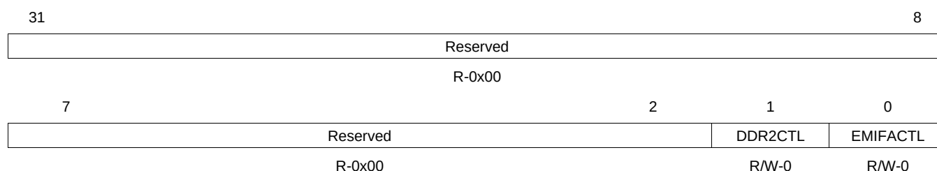
Figure 3-5. Peripheral Configuration Register 1 (PERCFG1) - 0x02AC 002C
