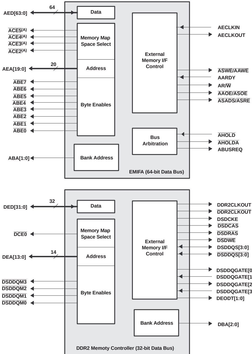
Figure 2-8. EMIFA/DDR2 Memory Controller Peripheral Signals
