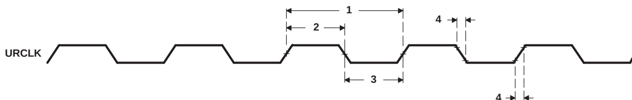
Figure 7-75. URCLK Timing
