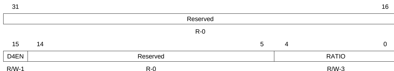
Figure 7-14. PLL Controller Divider 4 Register (PLLDIV4) [Hex Address: 029A 0160]
