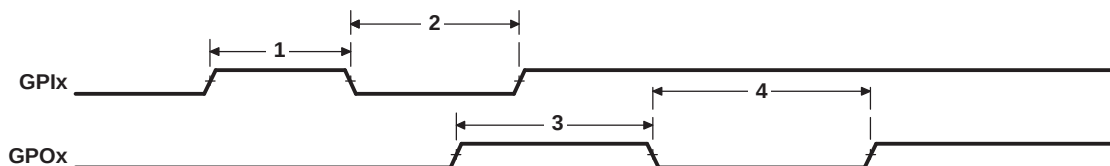
Figure 7-74. GPIO Port Timing
