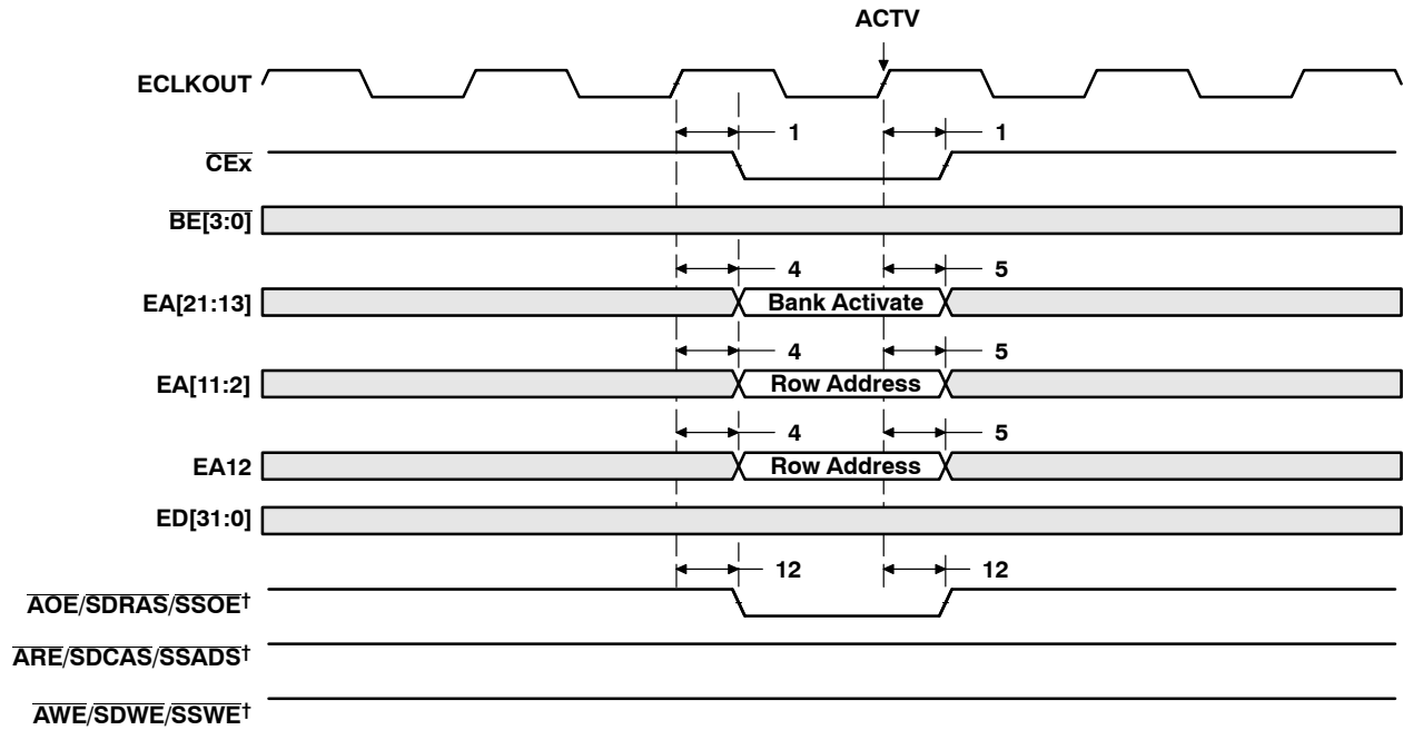
Figure 24. SDRAM ACTV Command
