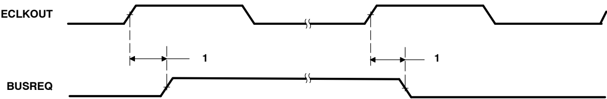
Figure 30. BUSREQ Timing
