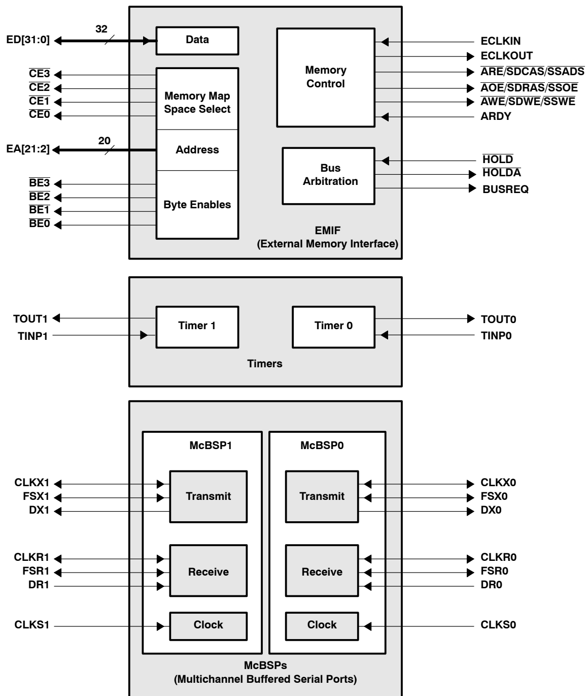
Figure 3. Peripheral Signals
