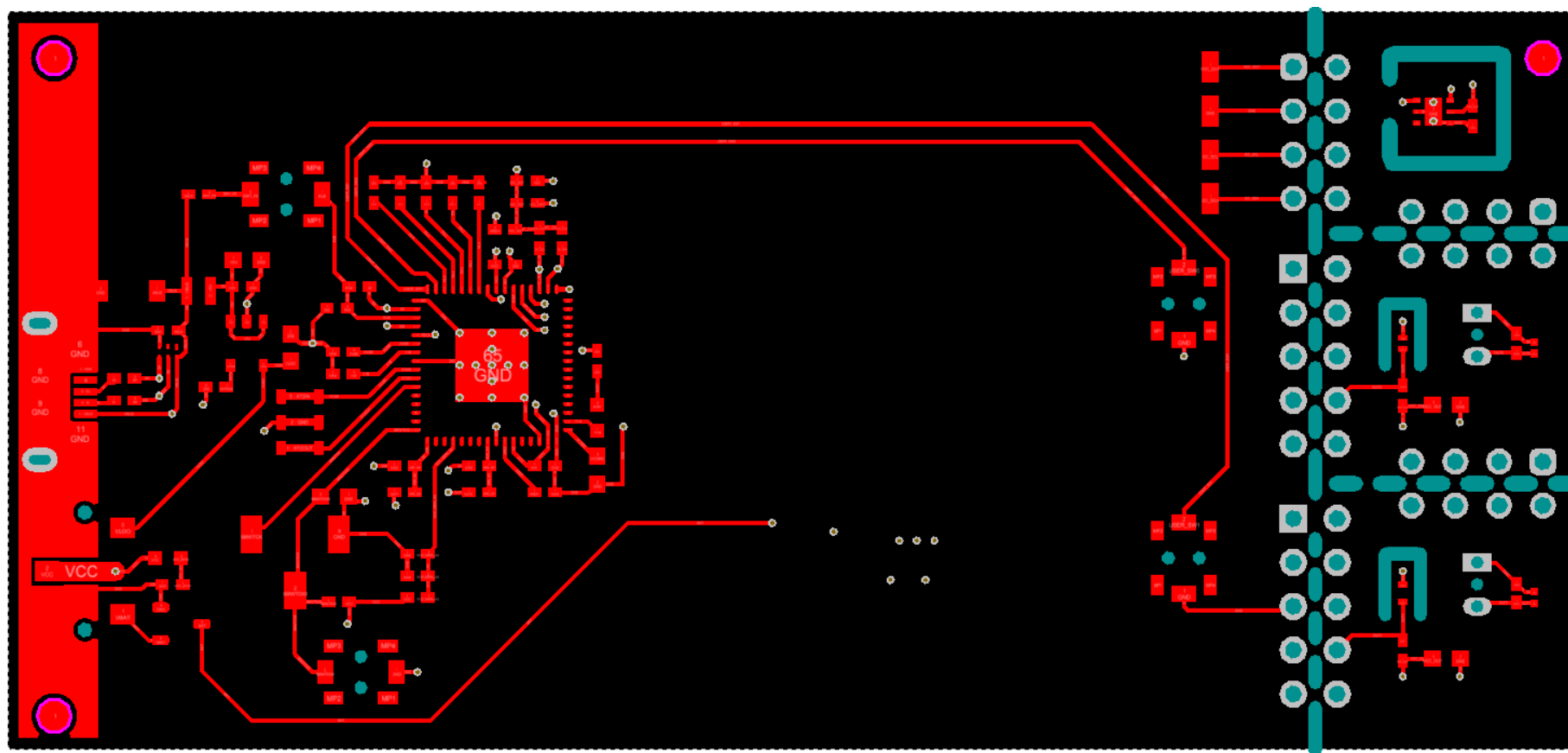
Figure 26. Top Signal Layer
