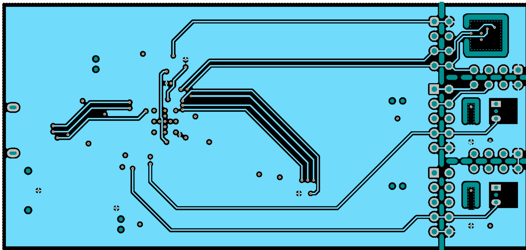
Figure 28. Power Layer
