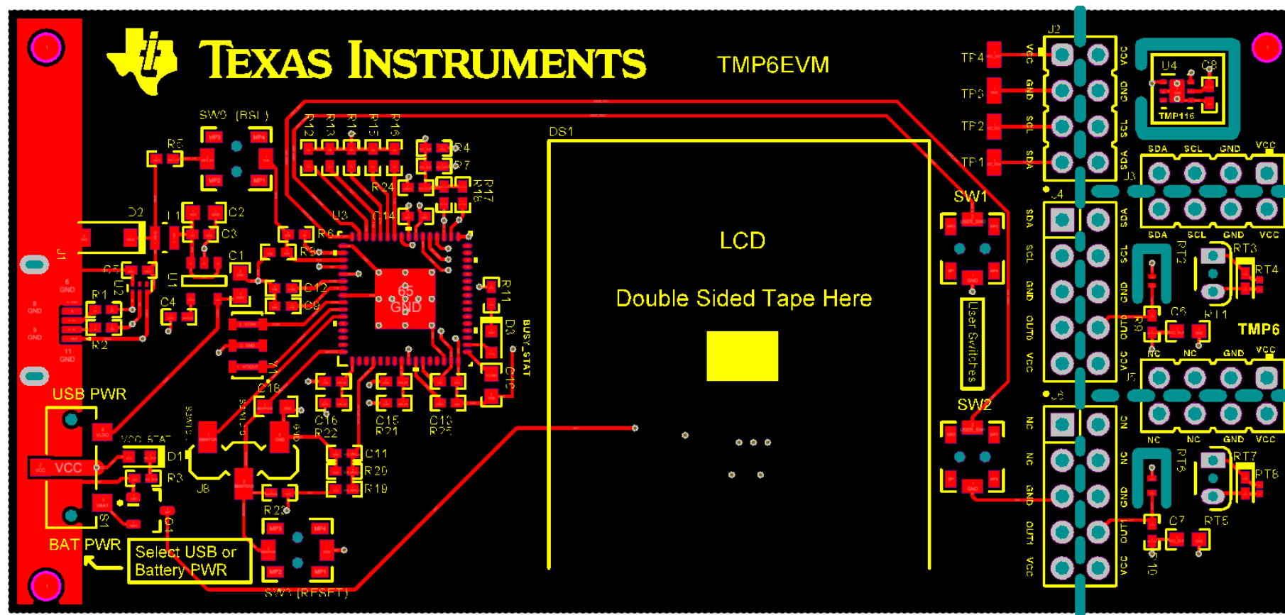
Figure 25. Top Layers
