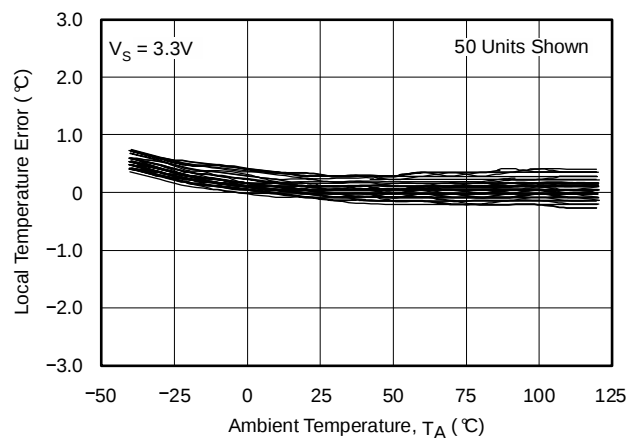
Figure 20. Local Temperature Error vs TMP411 Ambient Temperature
