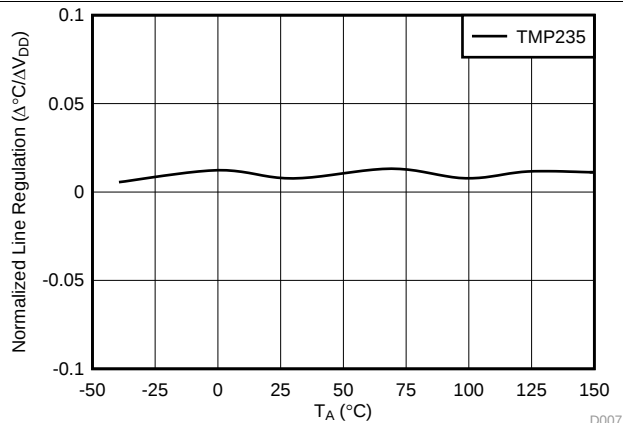
Figure 7. Line Regulation ( \Delta^\circ\text{C} / \Delta V_{\text{DD}} ) vs. Ambient Temperature
