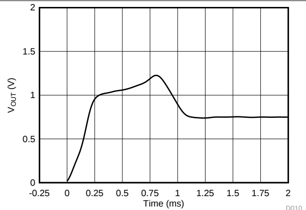
Figure 10. Output vs. Settling Time to Ramp V_{\text{DD}}
