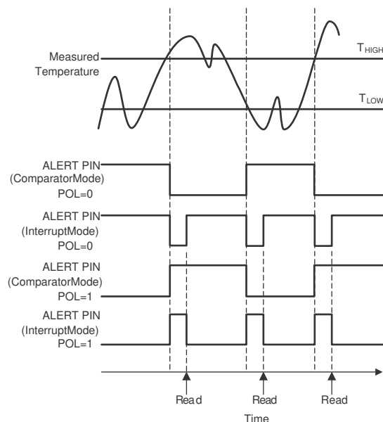
Figure 19. Output Transfer Function Diagrams
