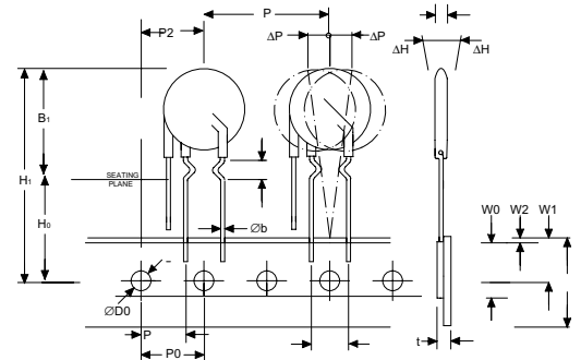
iTMOV varistor with inner crimp
