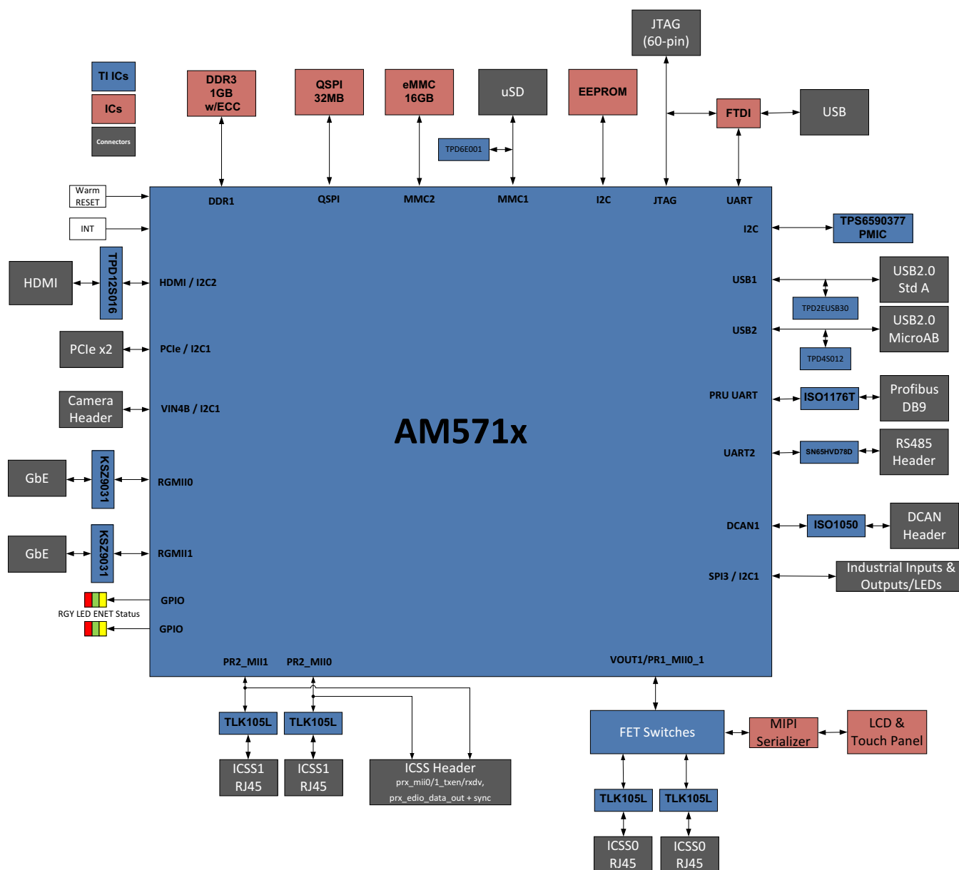
Figure 5. AM571x IDK EVM Block Diagram
