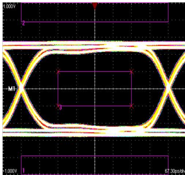
Figure 37. TMD5 Data Rate of 1856.25 Mbps
