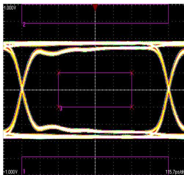
Figure 34. TMDS Data Rate of 1080 Mbps
