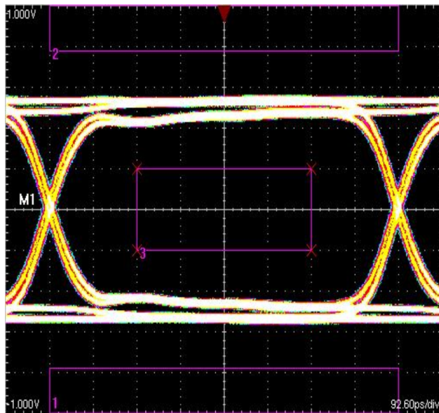
Figure 35. TMD5 Data Rate of 1350 Mbps
