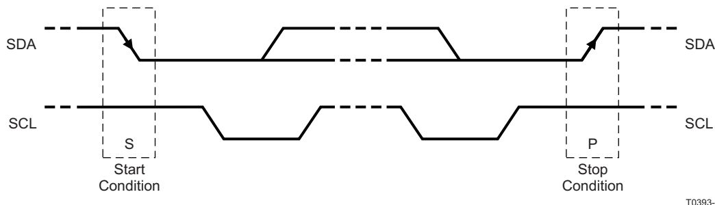
Figure 48. I²C Start and Stop Conditions
