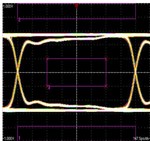
Figure 33. TMDS Data Rate of 847.5 Mbps
