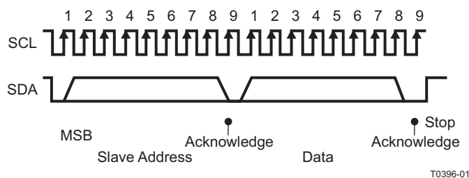
Figure 51. I²C Address, Data Cycle(s), and Stop
