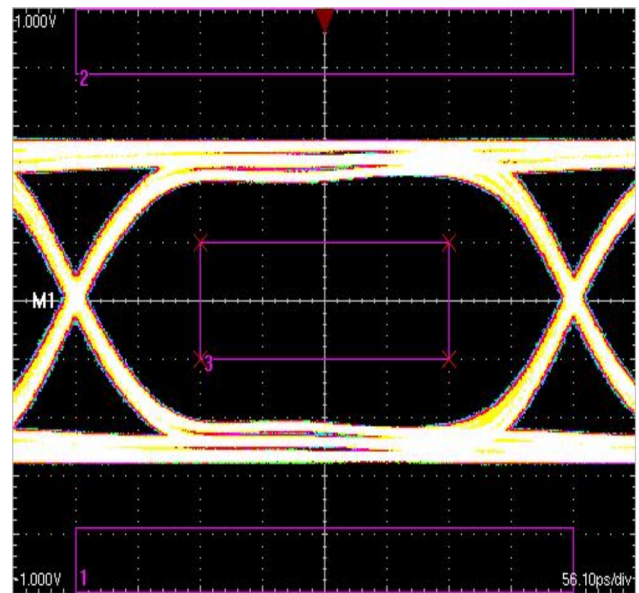
Figure 38. TMD5 Data Rate of 2227.5 Mbps
