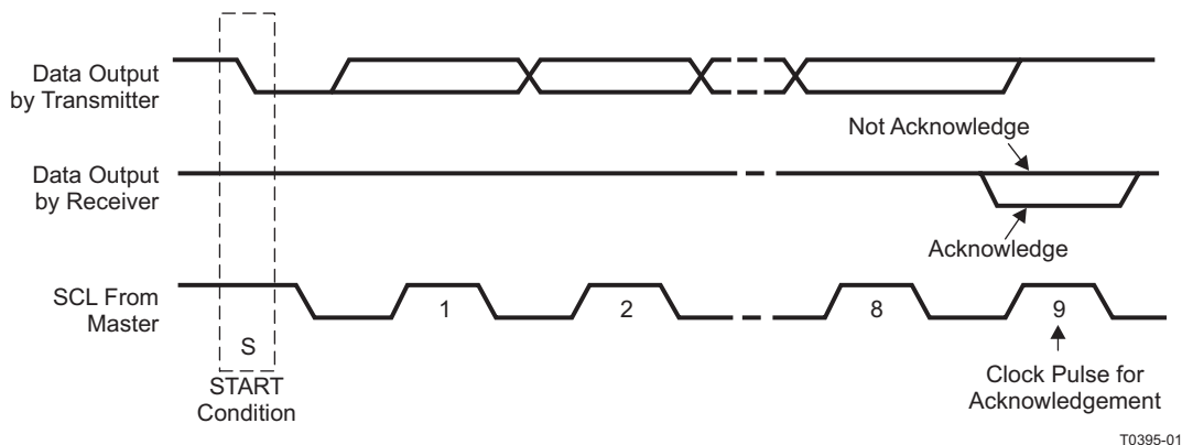
Figure 50. I²C Acknowledge
