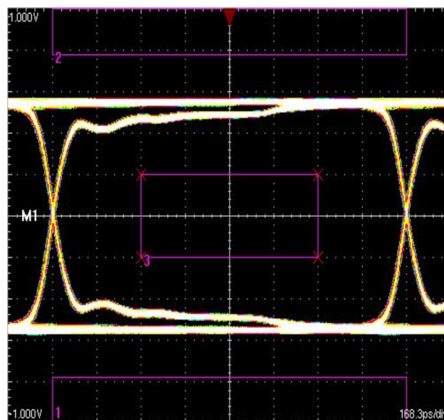
Figure 32. TMDS Data Rate of 742.5 Mbps
