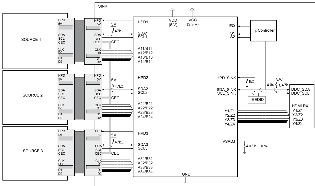
Figure 46. Three-Port HDMI-Enabled DTV With TMD5361B – CEC Commands Passing Through
