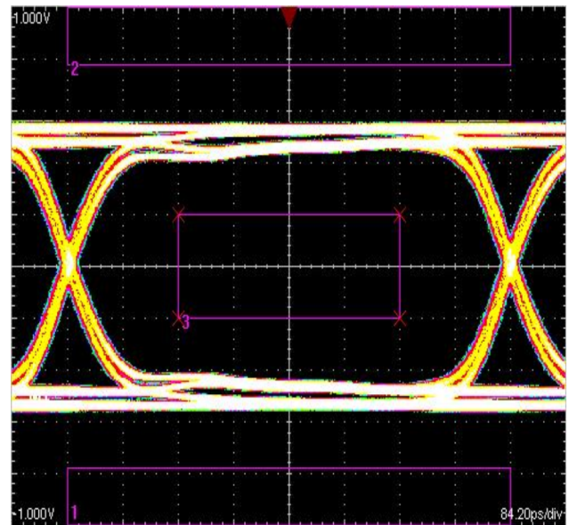
Figure 36. TMD5 Data Rate of 1485 Mbps
