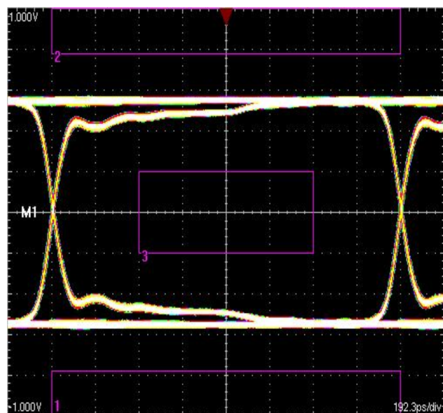
Figure 31. TMDS Data Rate of 650 Mbps
