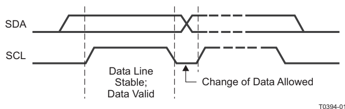
Figure 49. I²C Bit Transfer
