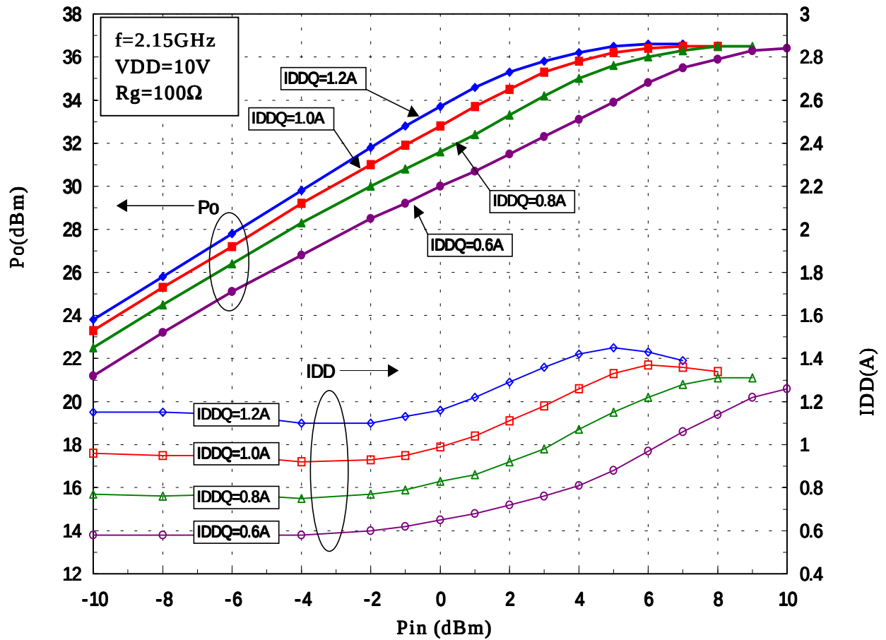
Output Power vs. Input Power
