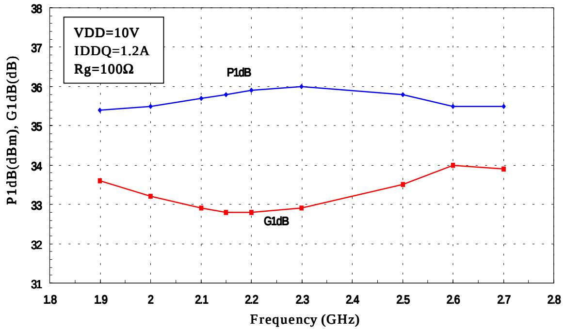
P1dB, G1dB vs. Frequency
