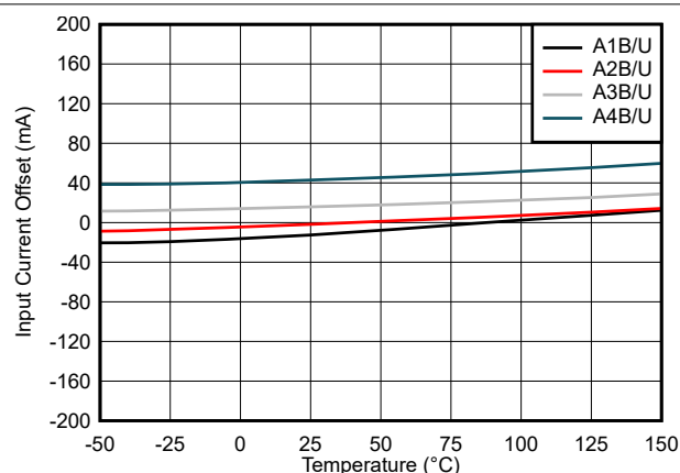
Figure 7-2. TMCS1107-Q1 Input Offset Current vs. Temperature
