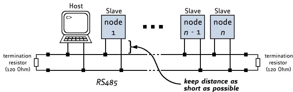
Figure 5.3: Bus structure
