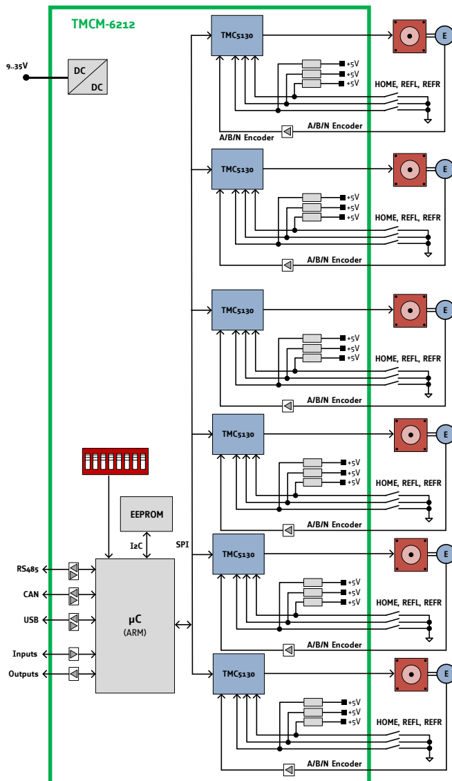
Figure 10.1 Main parts of the TCM-6212
