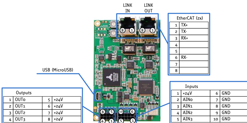
Figure 5.3 TMC6213 interface brick
