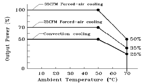
DERATING CURVE
