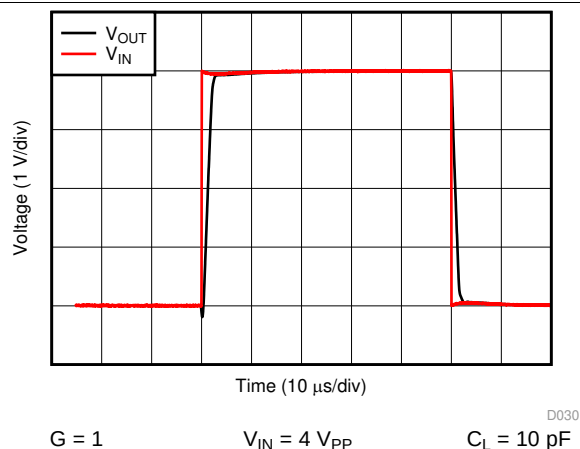
Figure 28. Overload Recovery
