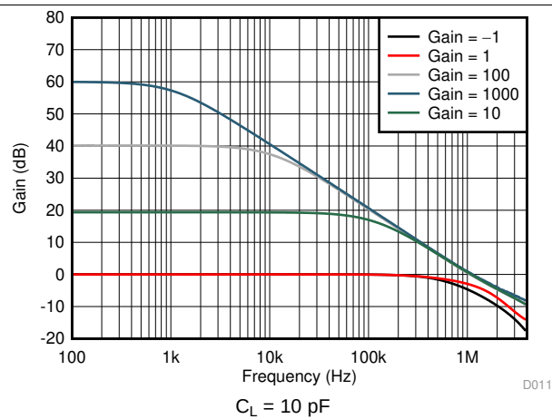
Figure 11. Closed-Loop Gain vs Frequency
