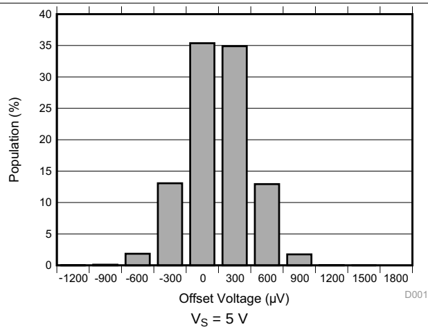
Figure 1. Offset Voltage Distribution Histogram
