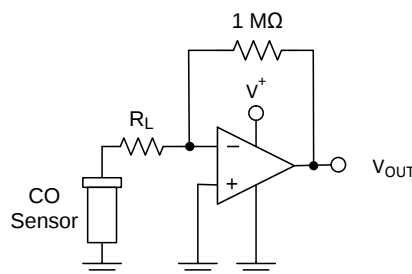
Nanopower CO Sensor
