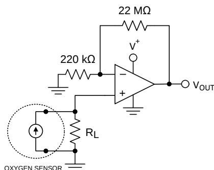
Nanopower Oxygen Sensor
