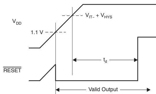
Figure 9. Power-Up Response
