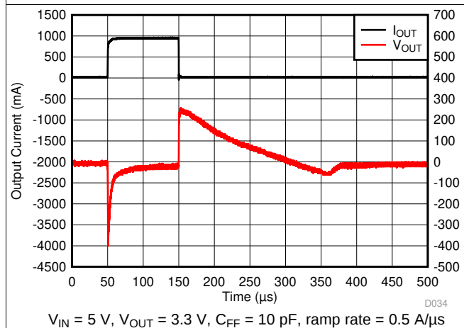
Figure 11. I_{OUT} Transient From 1 mA to 1 A
