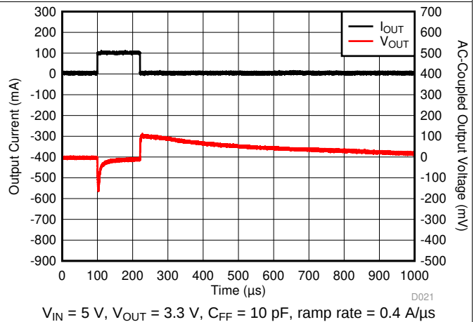
Figure 10. I_{OUT} Transient From 0 mA to 100 mA
