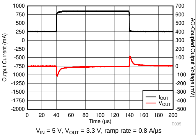
Figure 12. I_{OUT} Transient From 250 mA to 850 mA
