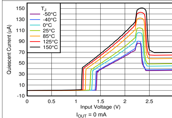
Figure 9. I_Q Increase Below Minimum V_{IN}
