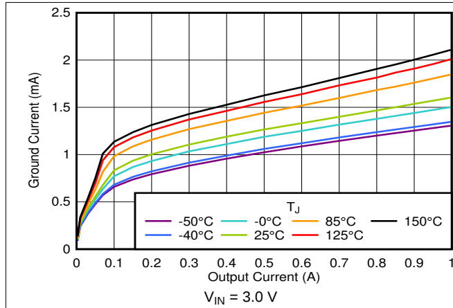
Figure 7. I_{GND} vs I_{OUT}
