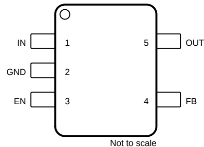
DBV Package (Preview) 5-Pin Adjustable SOT-23 Top View
