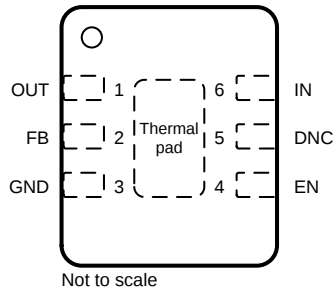
DRV Package 6-Pin Adjustable WSON Top View
