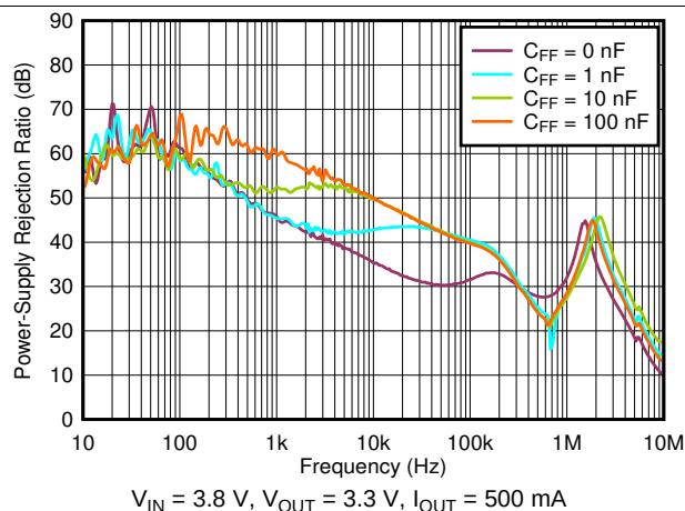
Figure 32. PSRR vs Frequency and C_{FF}
