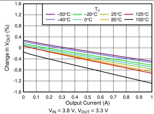
Figure 11. 3.3-V Load Regulation vs I_{OUT}
