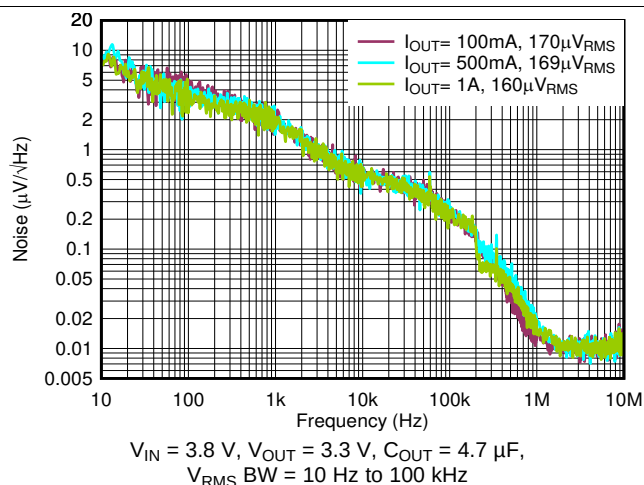
Figure 34. Output Spectral Noise Density vs Frequency
