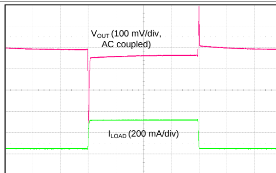
Figure 14. 1.0 V, 50-mA to 300-mA Load Transient
