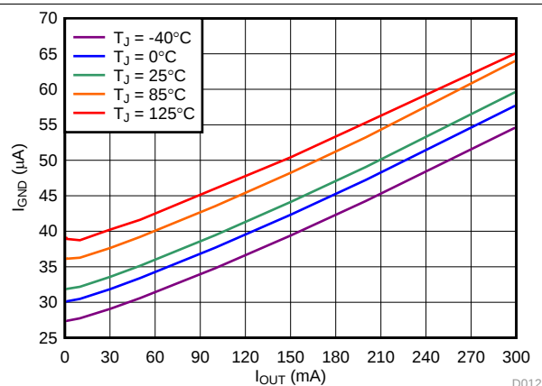
Figure 2. Ground Pin Current vs I_{OUT} and Temperature
