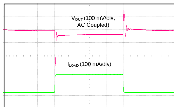
Figure 13. 1.0-V, 50-mA to 300-mA Load Transient
