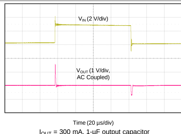
Figure 12. Line Transient
