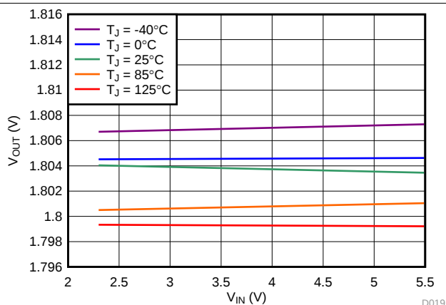
Figure 1. 1.8-V Regulation vs V_{IN} (Line Regulation) and Temperature
