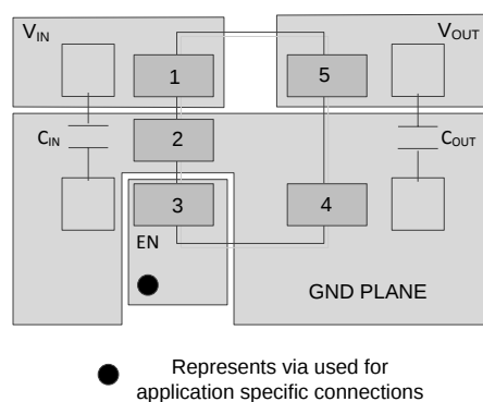
Figure 27. SOT-23 Layout Example
