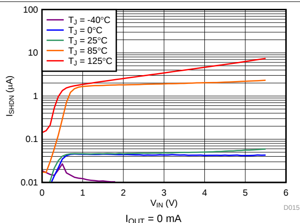
Figure 4. Shutdown Current vs V_{IN} and Temperature
