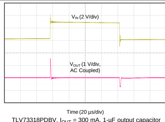
Figure 24. Line Transient
