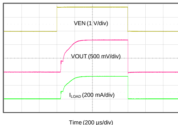
Figure 1. Startup Performance with a 3.7- \Omega Load Resistor, VIN = 1.8 V
