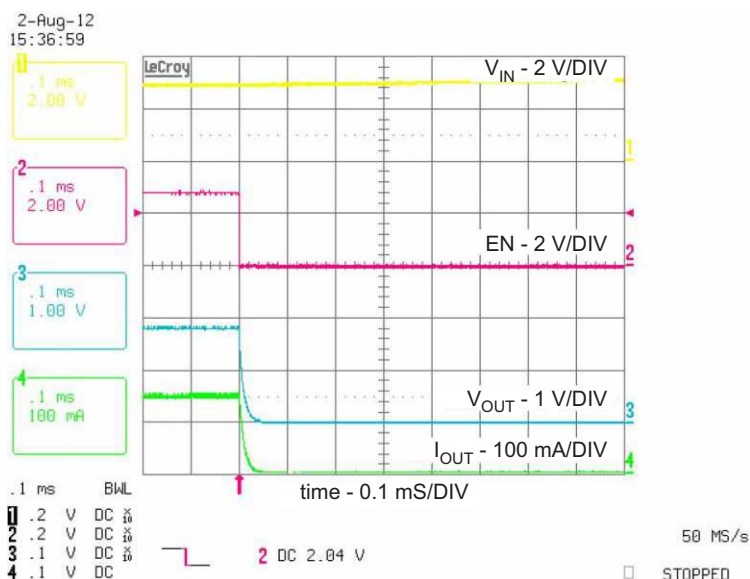
Figure 2. Turn-off Waveforms of the TLV71318PEVM-171
