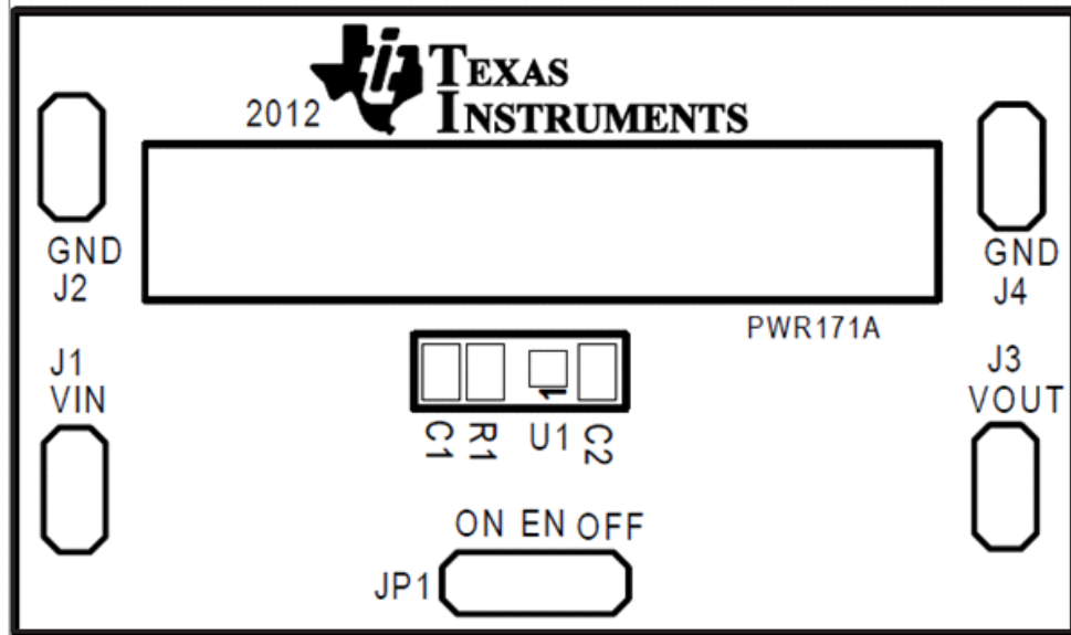
Figure 6. Assembly Layer
