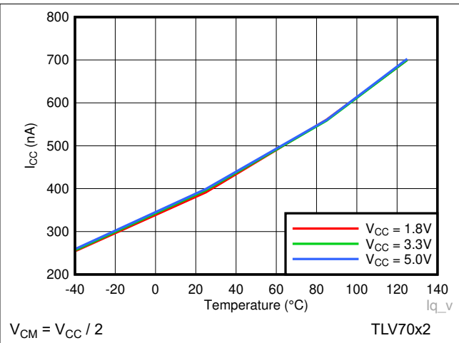
Figure 6-22. I_{CC} vs Temperature
