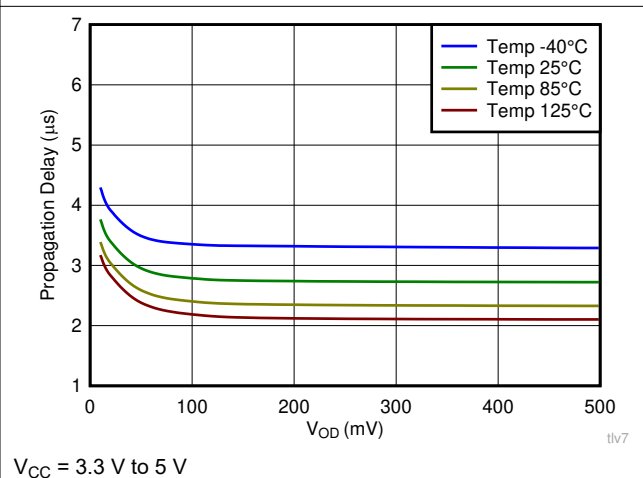
Figure 6-26. Propagation Delay (H-L) vs Input Overdrive
