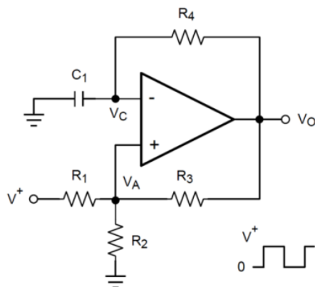
Figure 40. Square-Wave Oscillator
