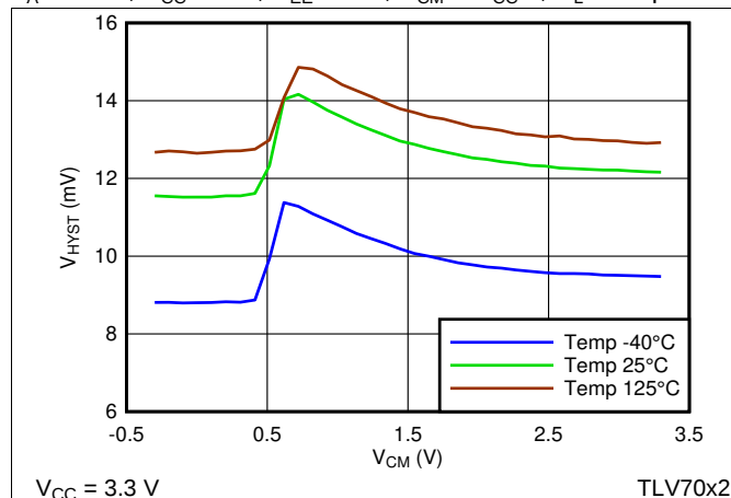
Figure 15. Hysteresis vs V_{CM}
