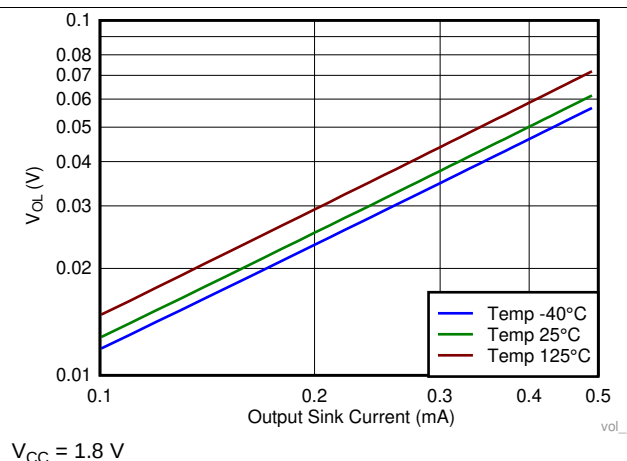
Figure 20. Output Voltage Low vs Output Sink Current
