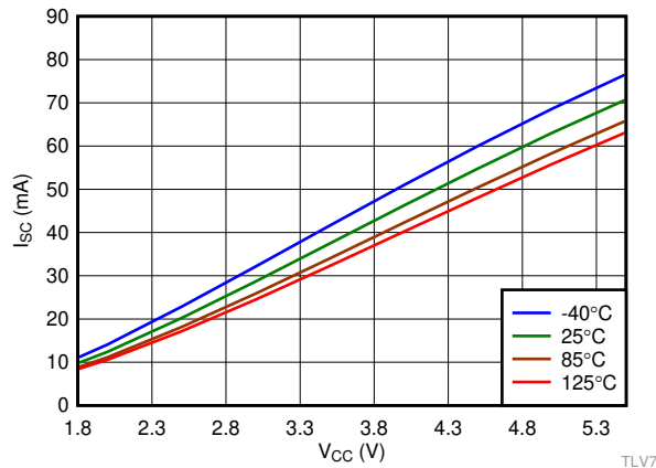
Figure 21. TLV701x Output Short Circuit (Source) vs. V_{CC}
