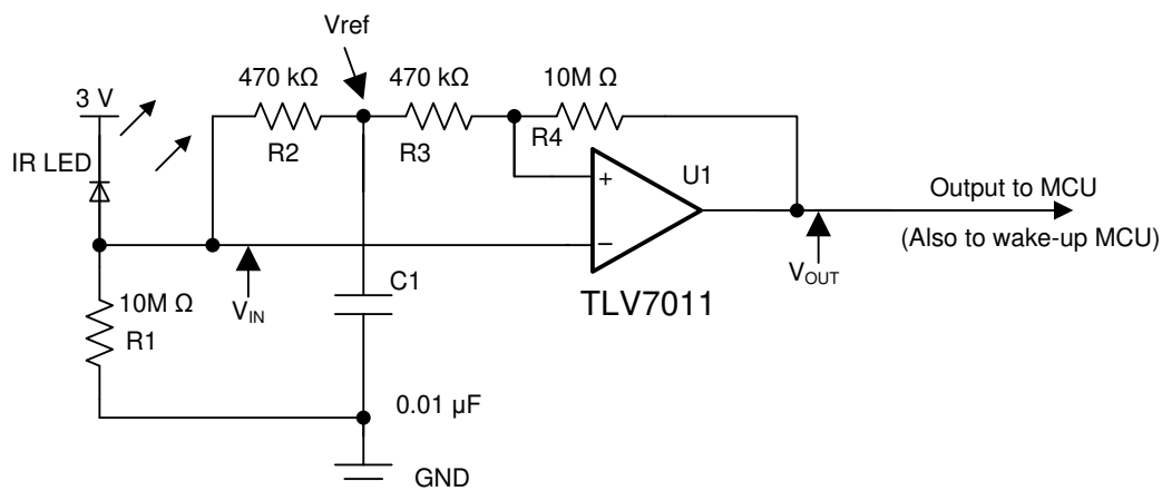
Figure 37. IR Receiver Analog Front End Using TLV7011
