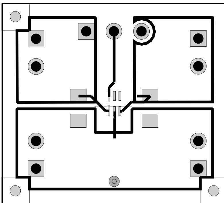
Figure 2. Top Layer Routing
