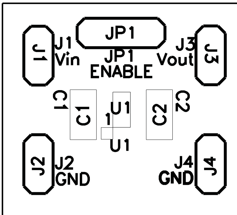
Figure 1. Assembly Layer
