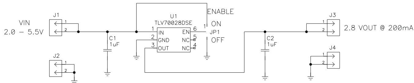
Figure 4. TLV700xxEVM-463 Schematic
