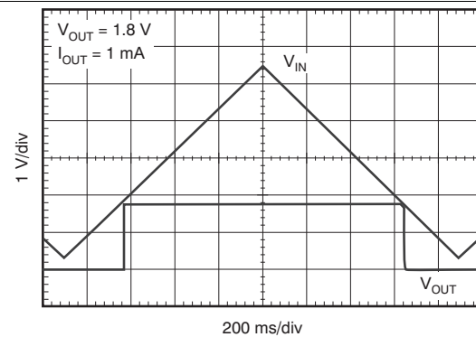
Figure 20. V_{IN} Ramp Up, Ramp Down Response
