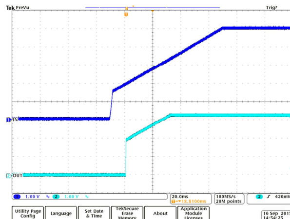
Figure 22. Power Up
