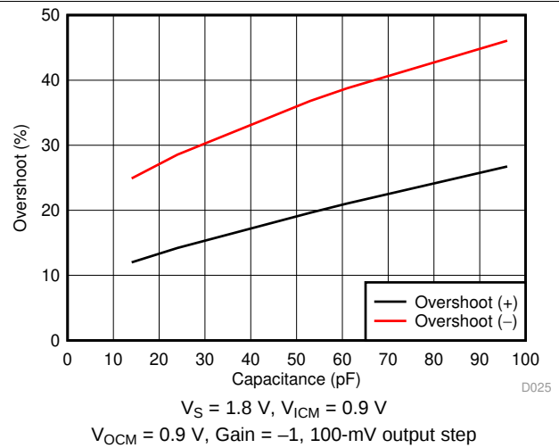
Figure 28. Small-Signal Overshoot vs Load Capacitance
