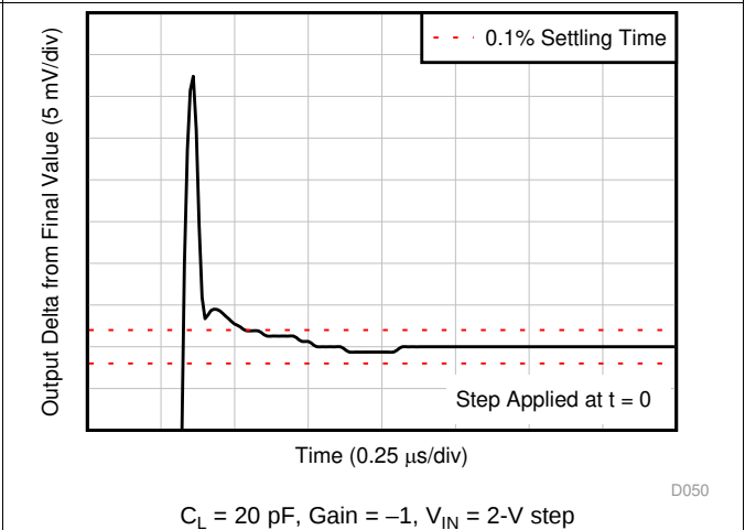
Figure 68. Large Signal Settling Time (Negative)
