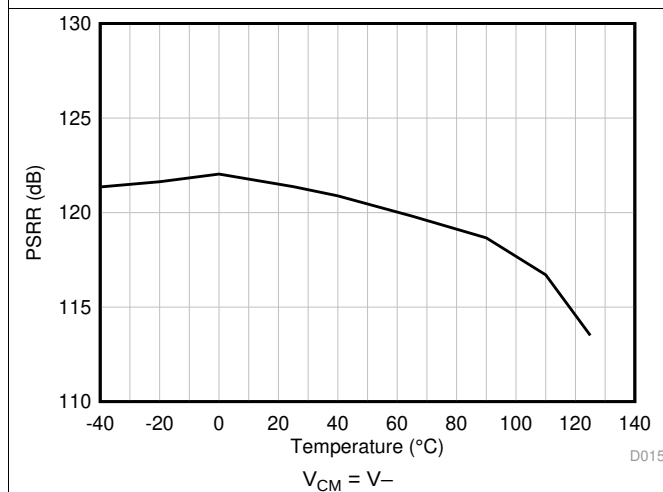
Figure 53. PSRR vs Temperature
