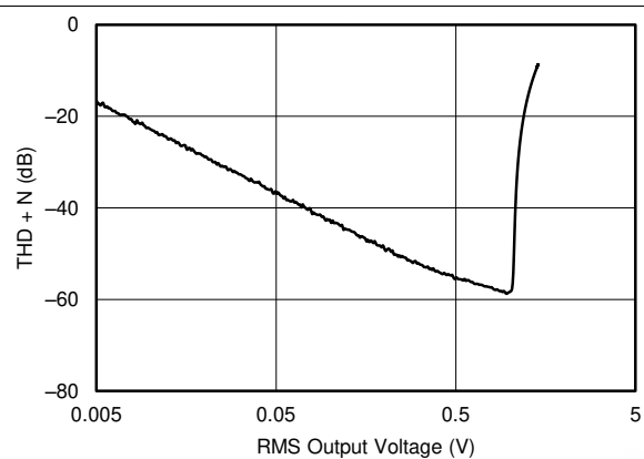
Figure 87. THD + N vs RMS Output Voltage
