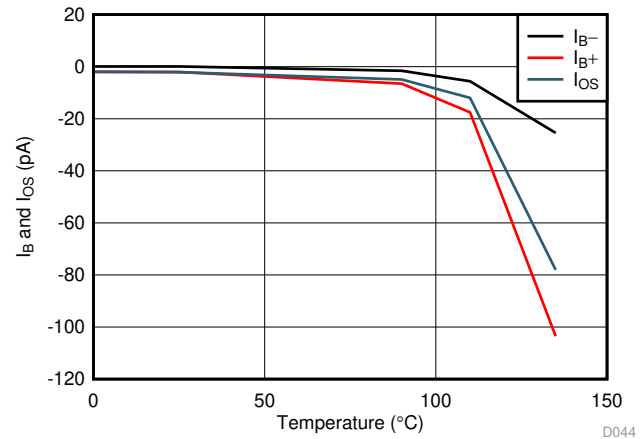
Figure 8. I_B and I_{OS} vs Temperature
