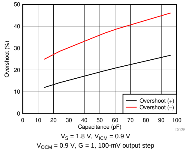
Figure 26. Small-Signal Overshoot vs Load Capacitance
