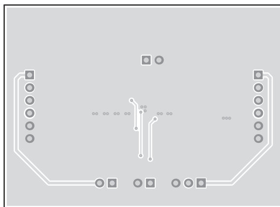
Figure 2. Bottom Layer
