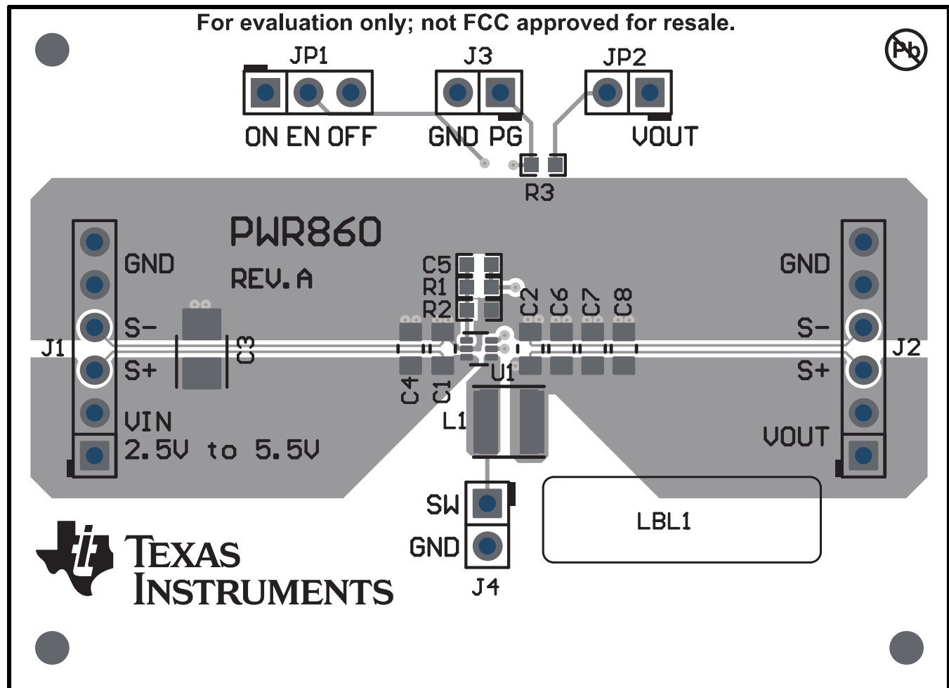
Figure 1. Top Layer
