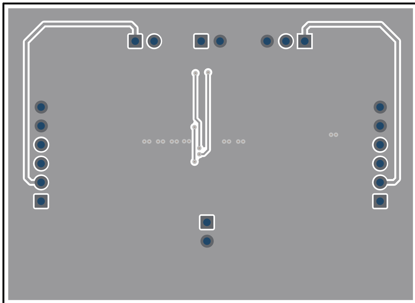
Figure 2. Bottom Layer
