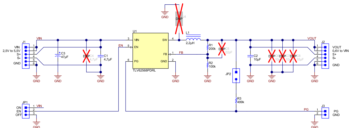
Figure 3. TLV6256xEVM-860 Schematic
