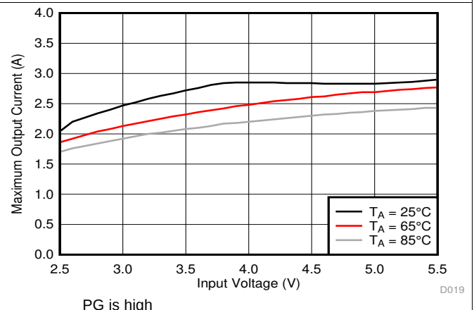
Figure 16. Maximum Output Current at V_{OUT} = 1.8\text{ V}
